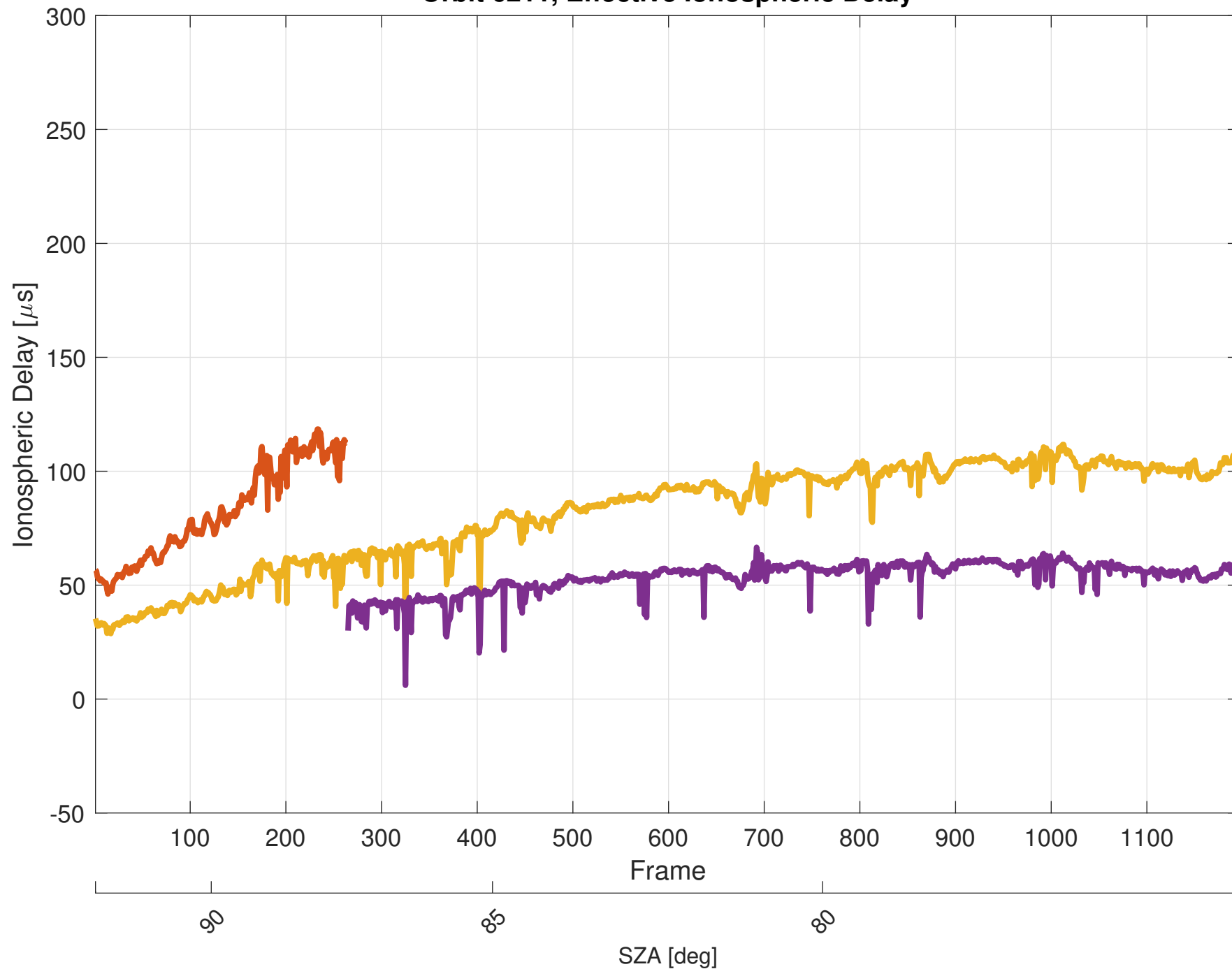
Orbit 6211, Effective Ionospheric Delay
