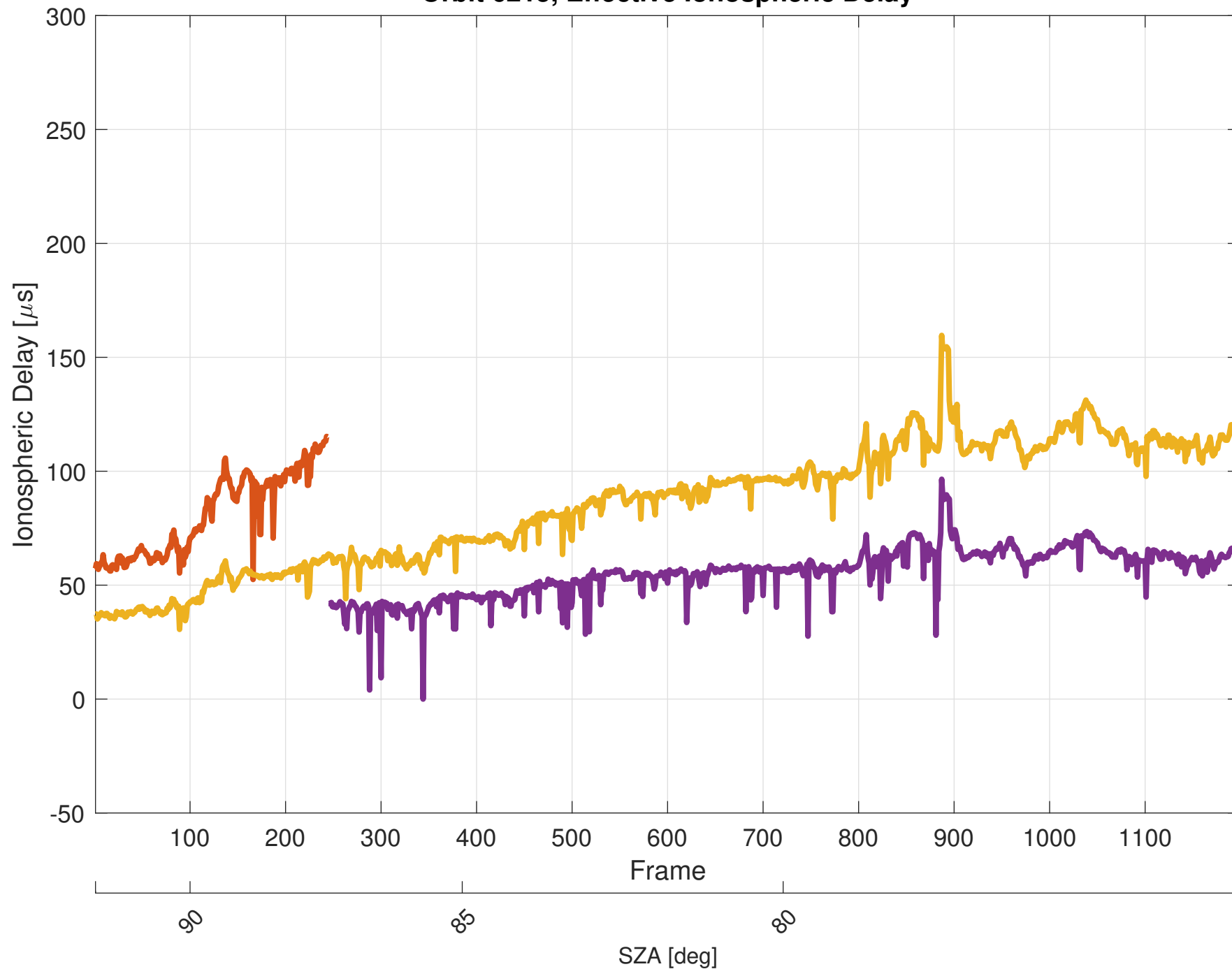
Orbit 6215, Effective Ionospheric Delay
