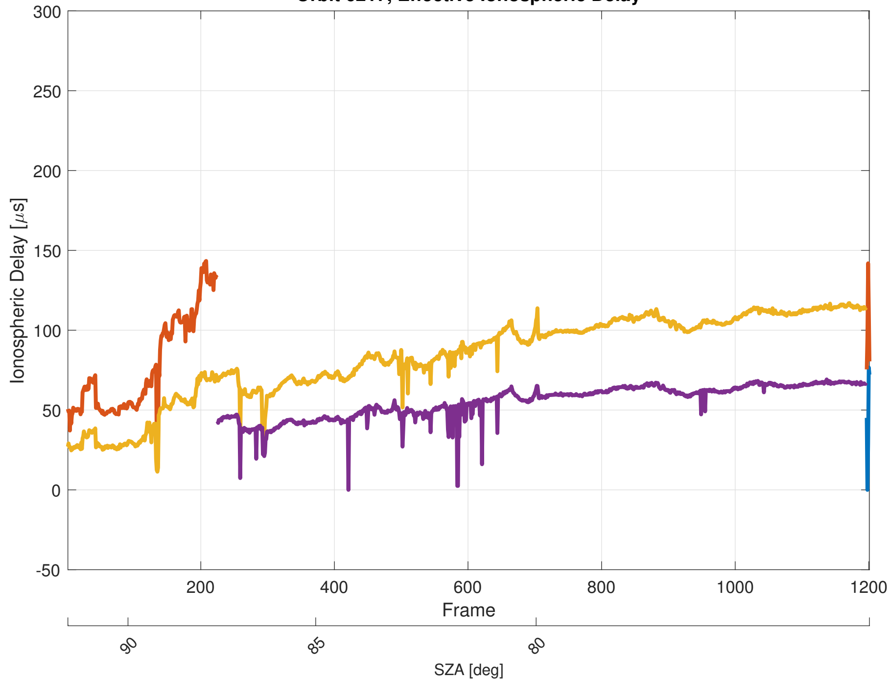
Orbit 6217, Effective Ionospheric Delay
