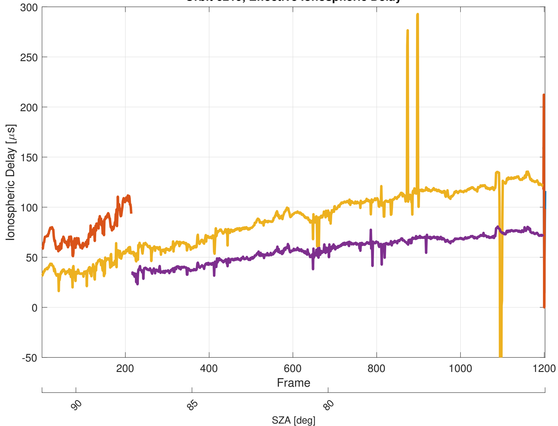
Orbit 6219, Effective Ionospheric Delay
