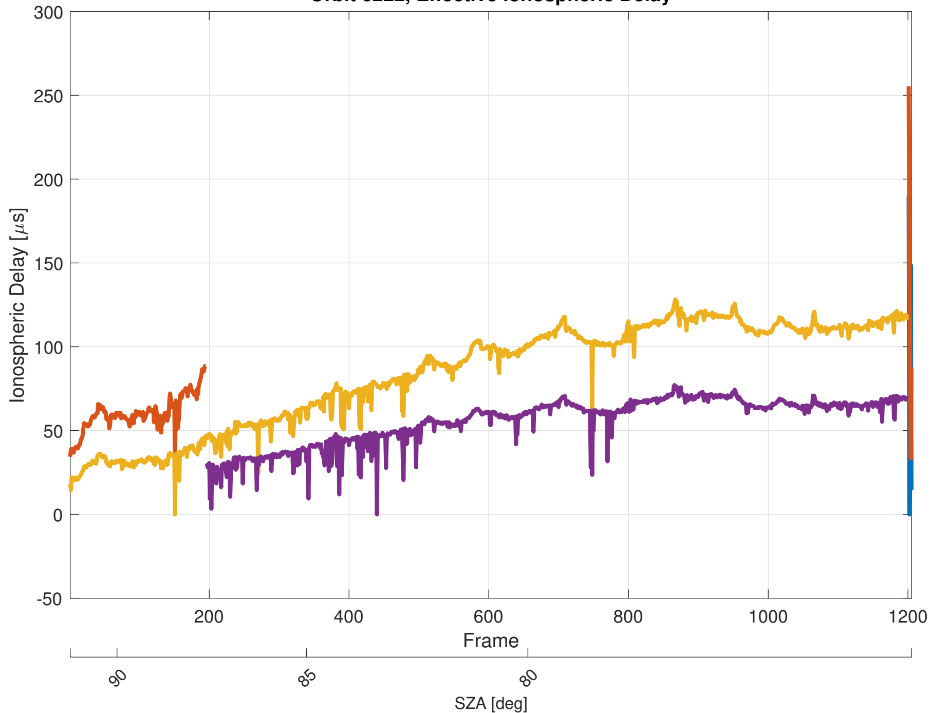
Orbit 6222, Effective Ionospheric Delay
