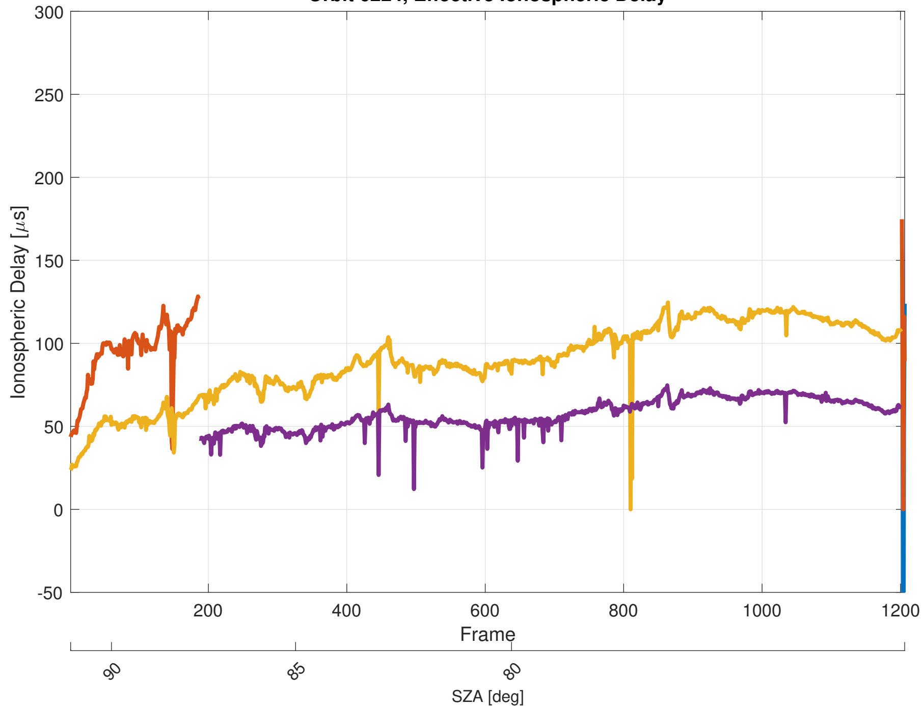
Orbit 6224, Effective Ionospheric Delay
