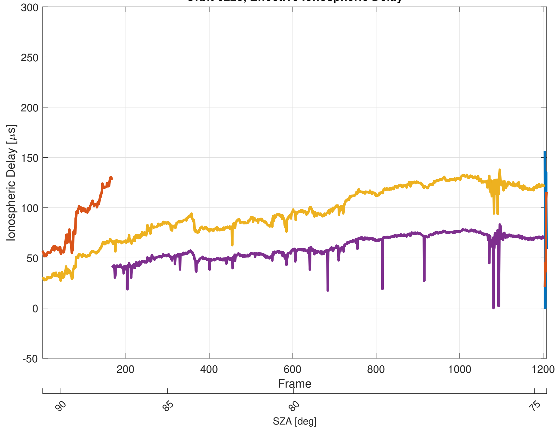
Orbit 6228, Effective Ionospheric Delay
