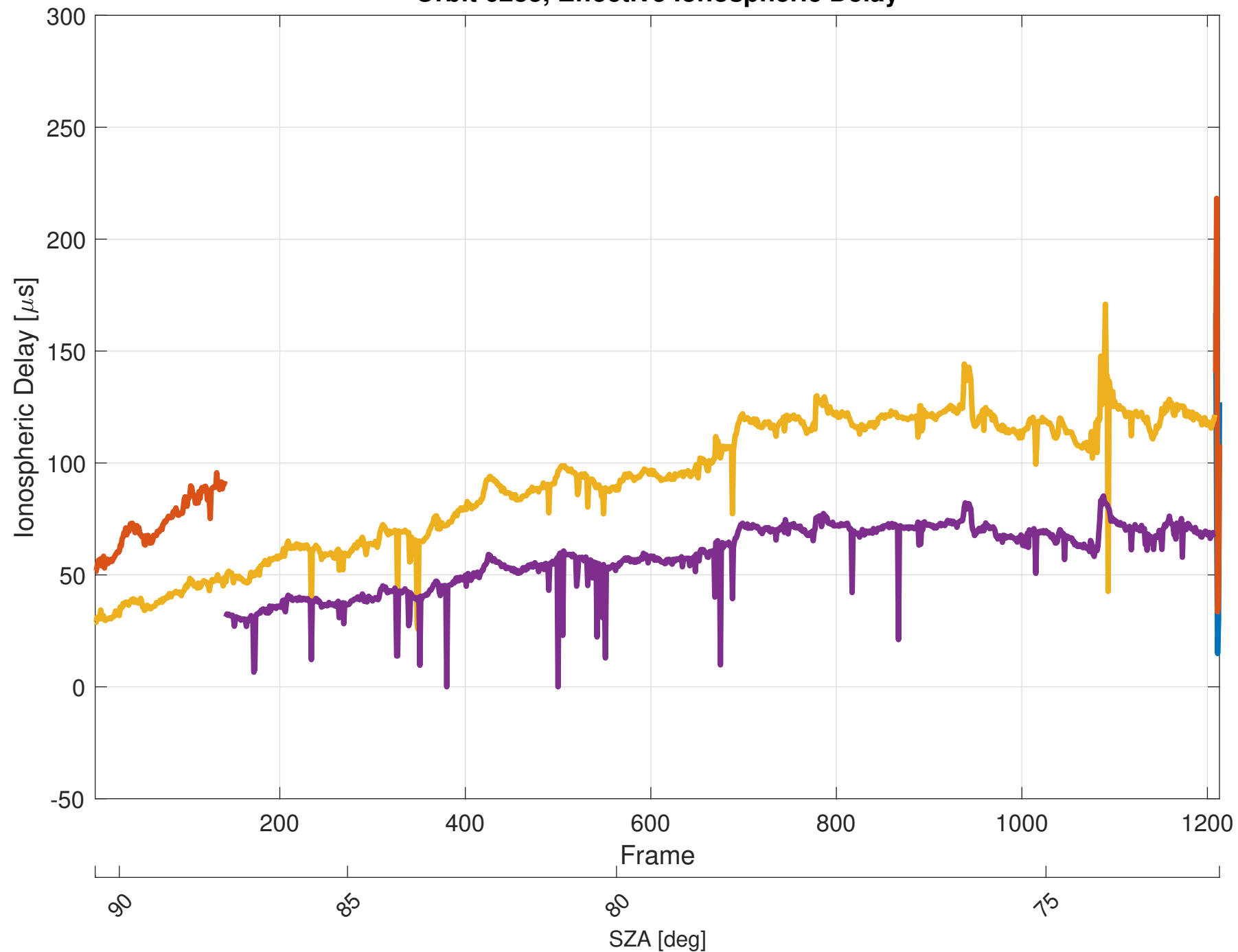
Orbit 6233, Effective Ionospheric Delay
