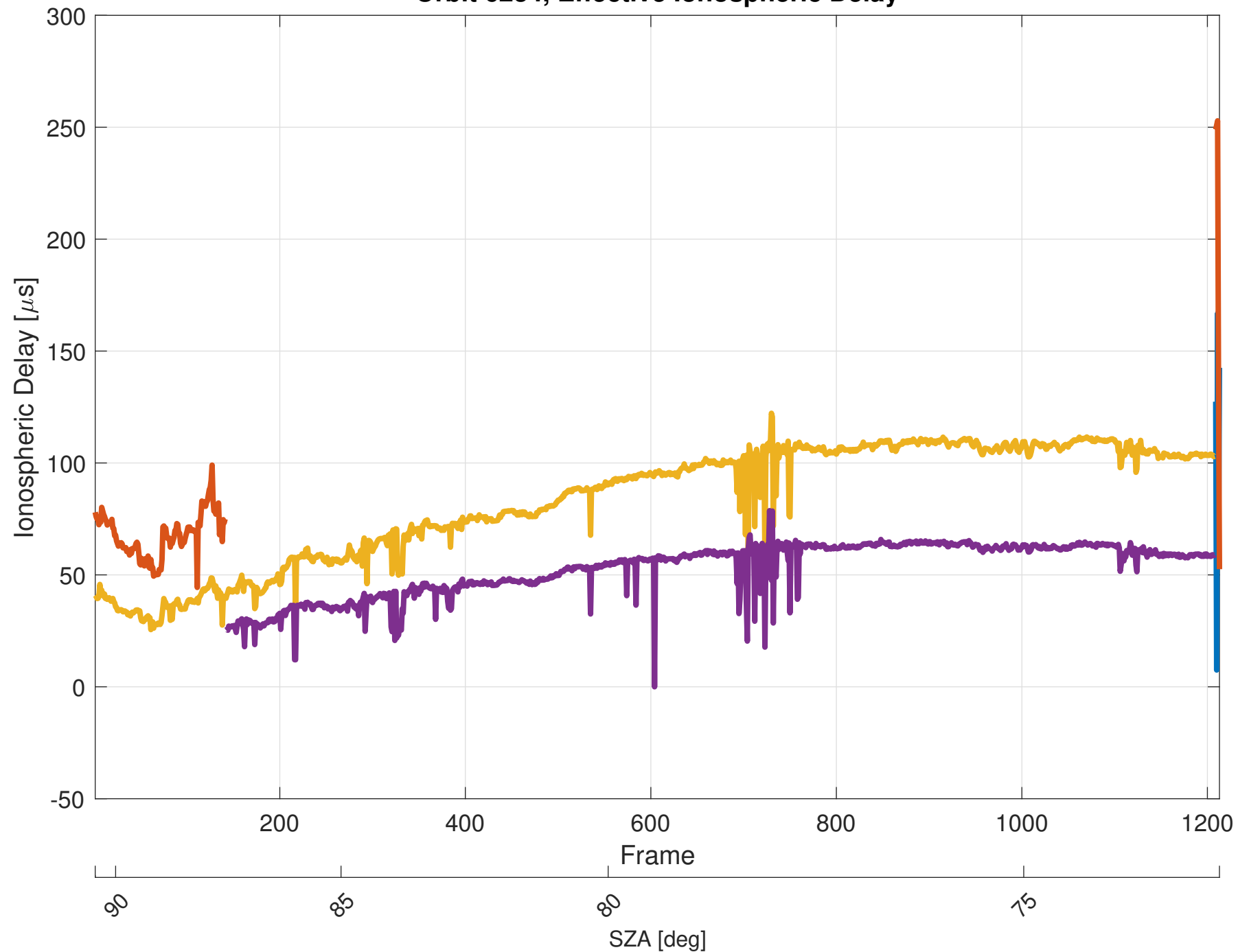
Orbit 6234, Effective Ionospheric Delay
