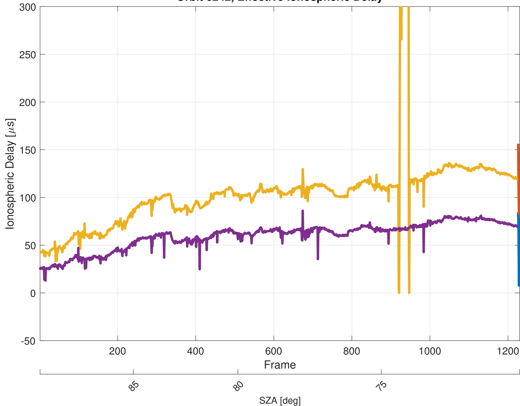
Orbit 6242, Effective Ionospheric Delay
