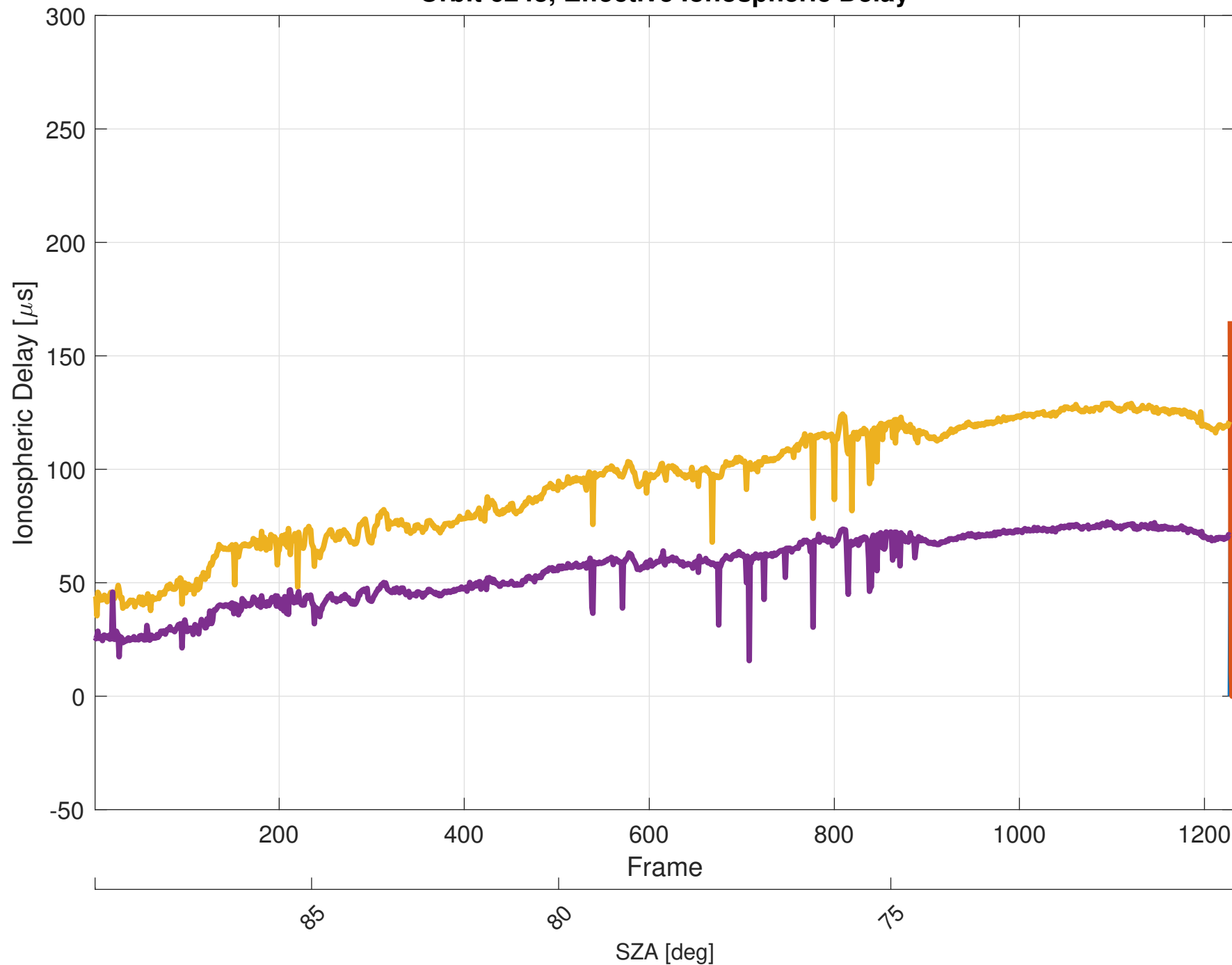
Orbit 6243, Effective Ionospheric Delay
