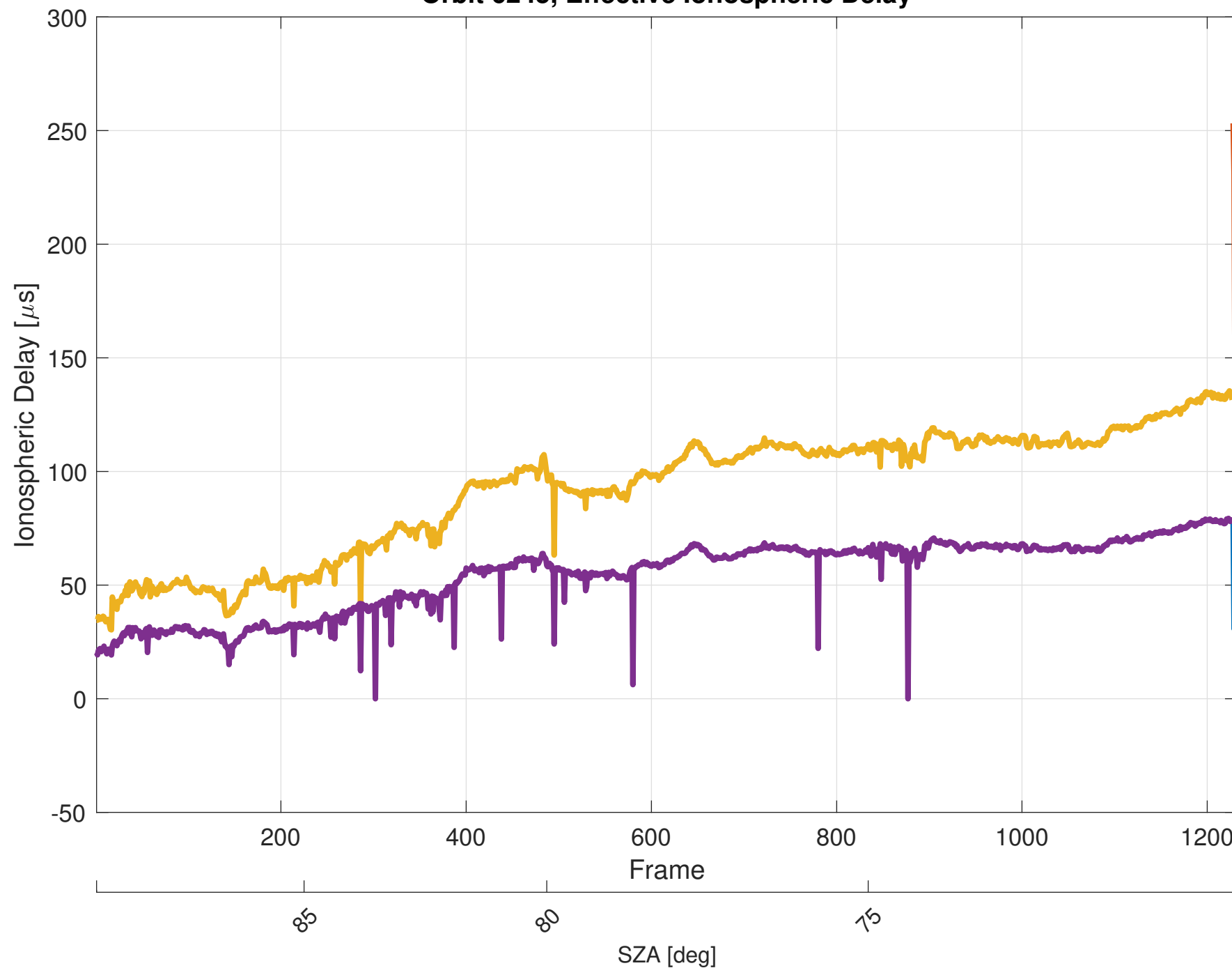
Orbit 6245, Effective Ionospheric Delay
