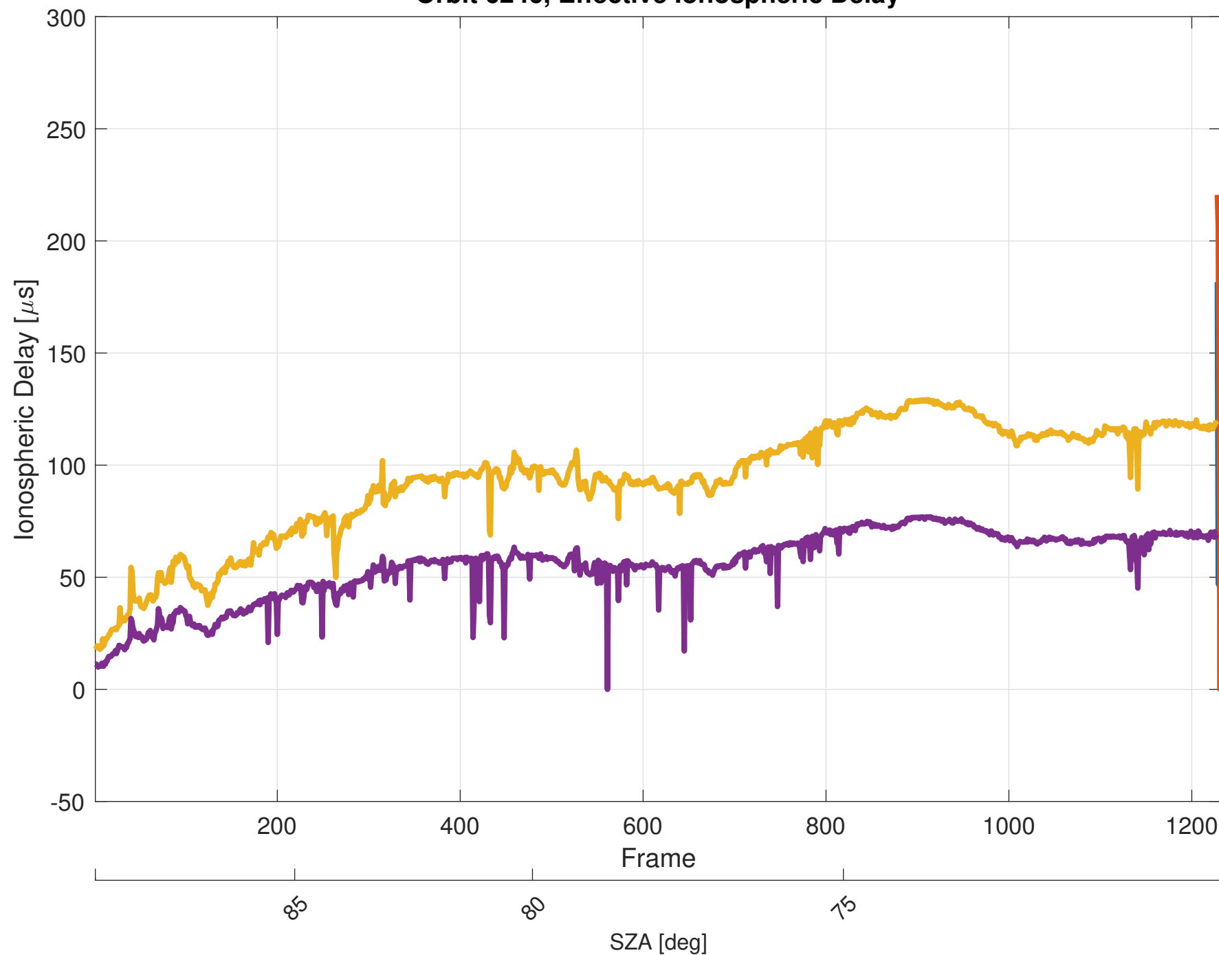
Orbit 6246, Effective Ionospheric Delay
