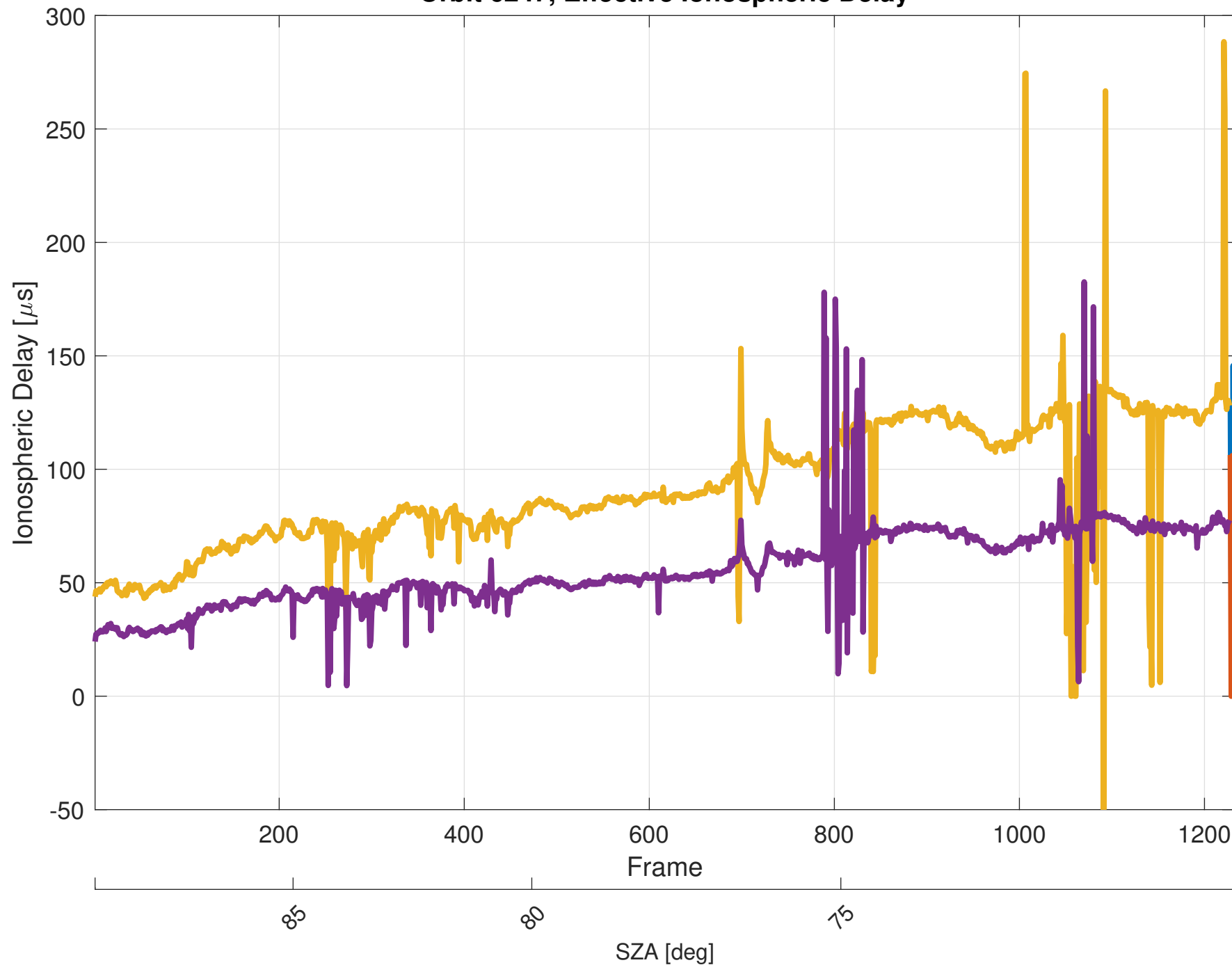
Orbit 6247, Effective Ionospheric Delay
