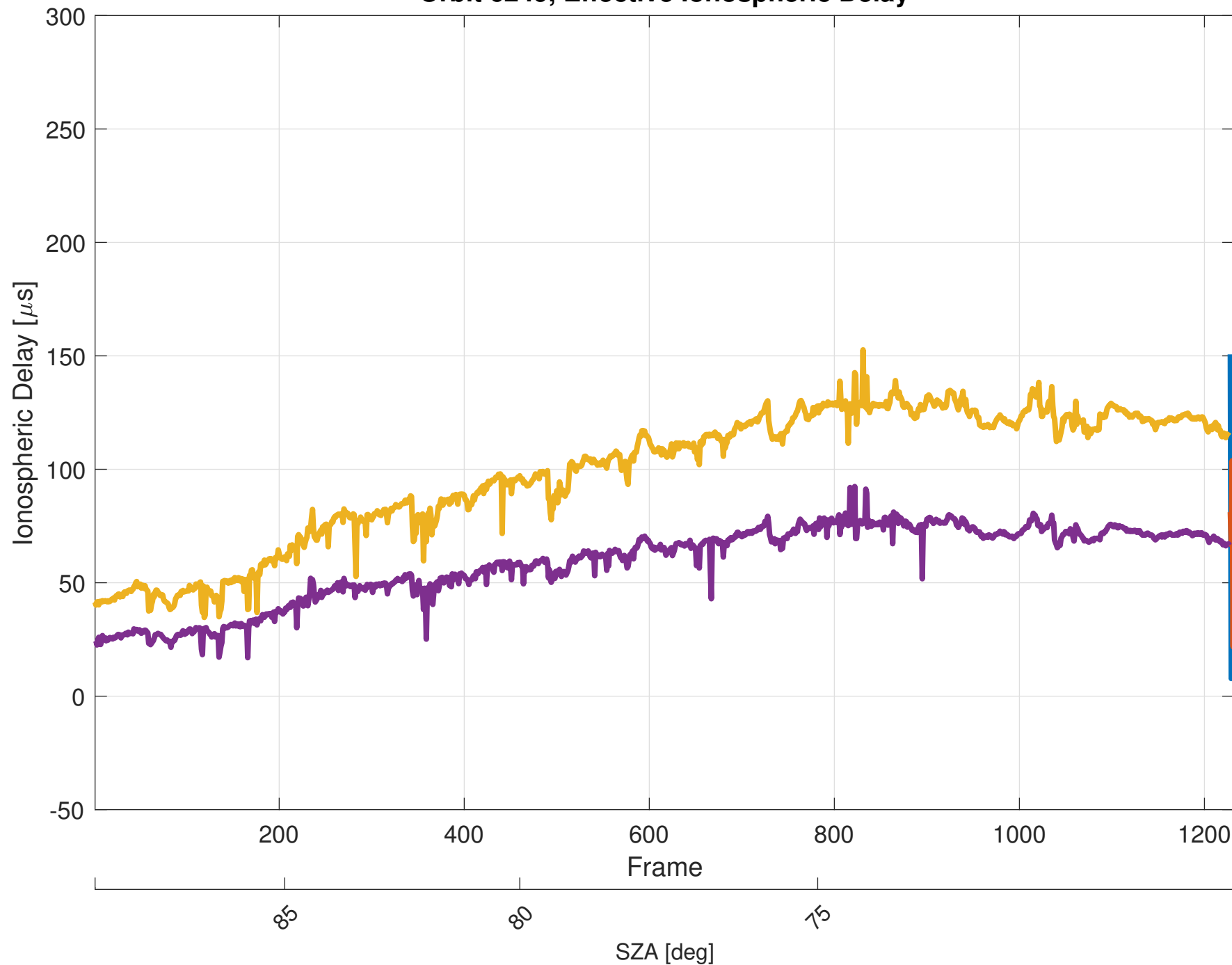
Orbit 6249, Effective Ionospheric Delay
