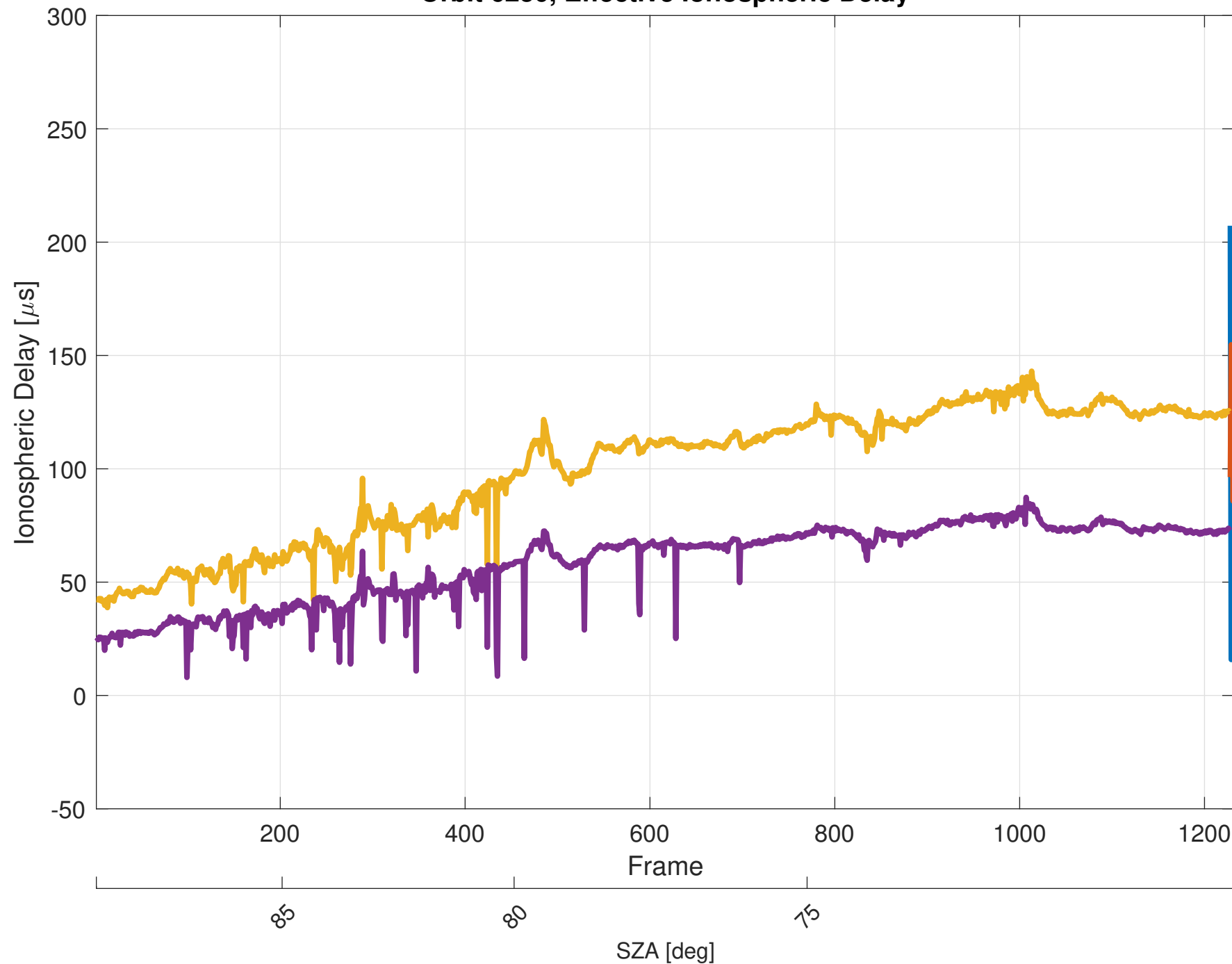
Orbit 6250, Effective Ionospheric Delay
