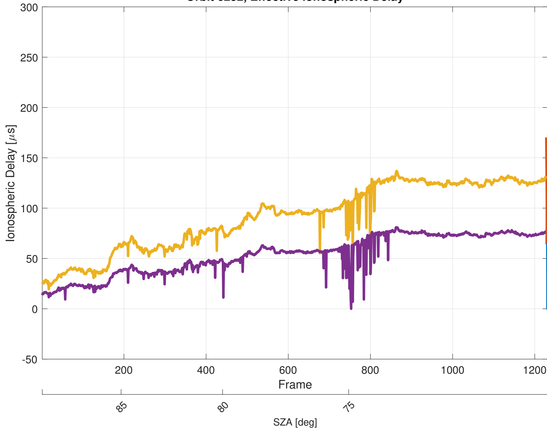
Orbit 6252, Effective Ionospheric Delay
