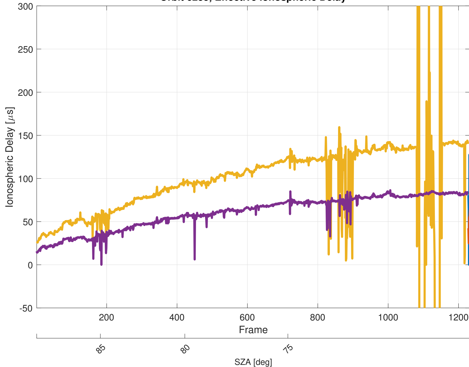
Orbit 6255, Effective Ionospheric Delay
