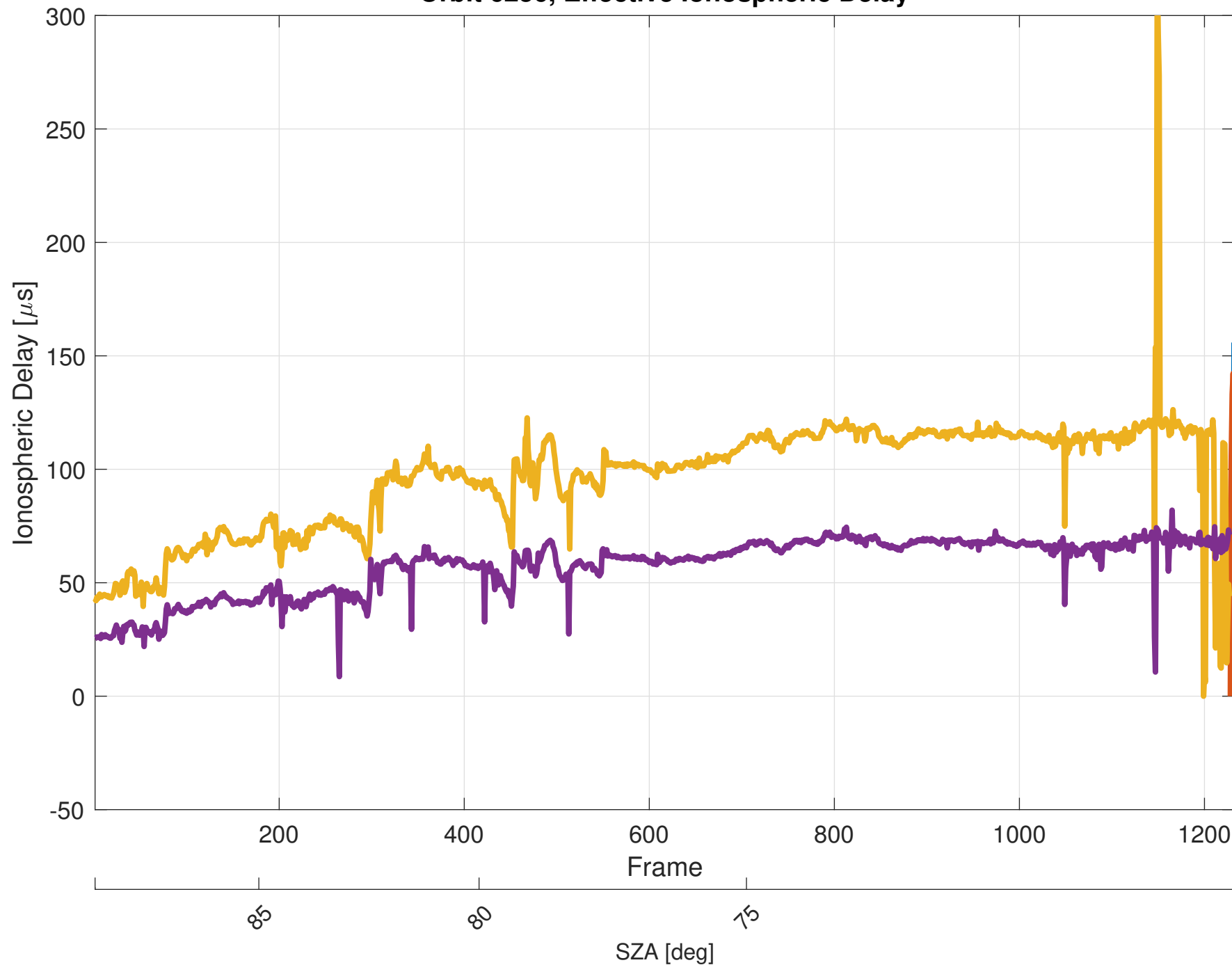
Orbit 6256, Effective Ionospheric Delay
