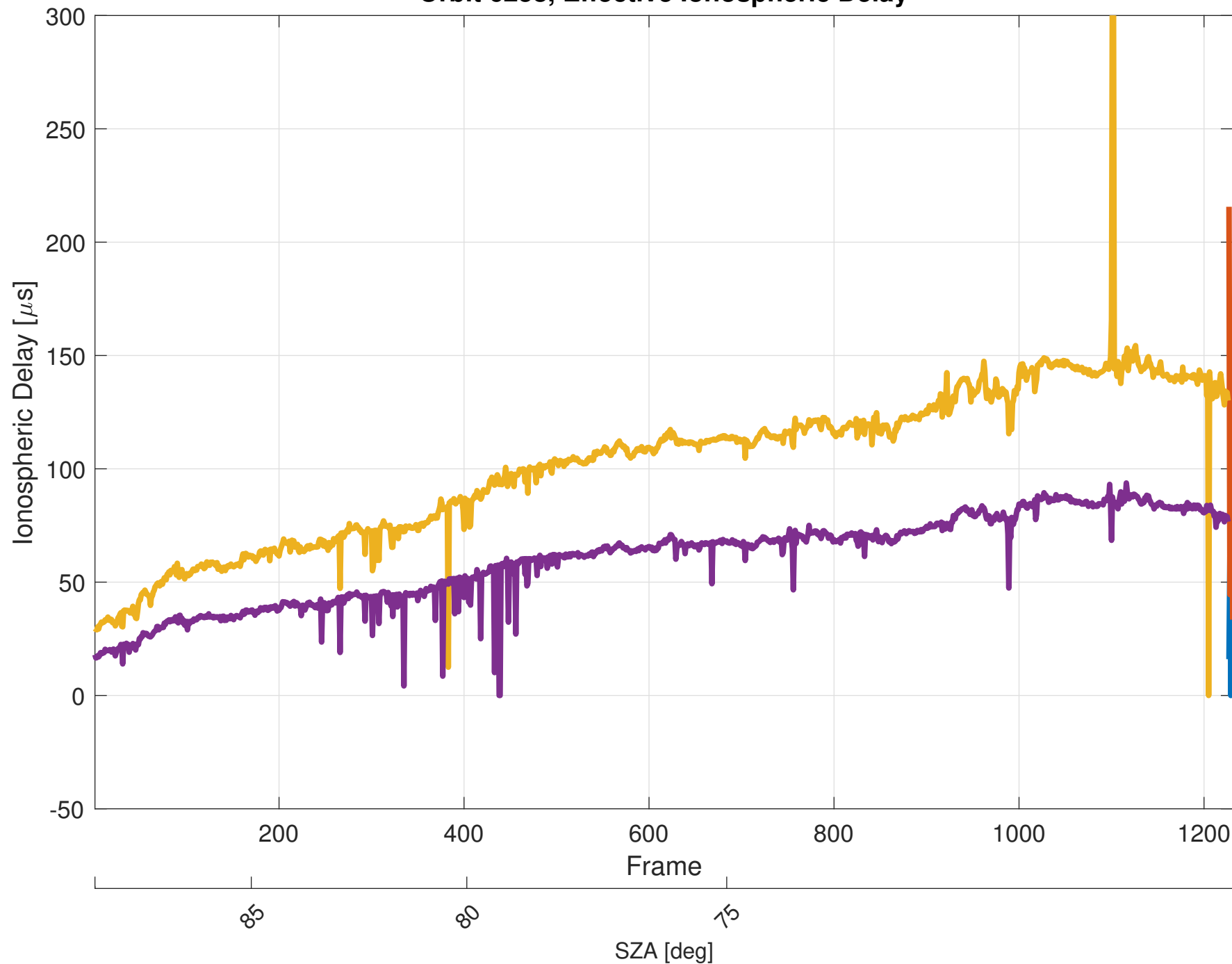
Orbit 6258, Effective Ionospheric Delay
