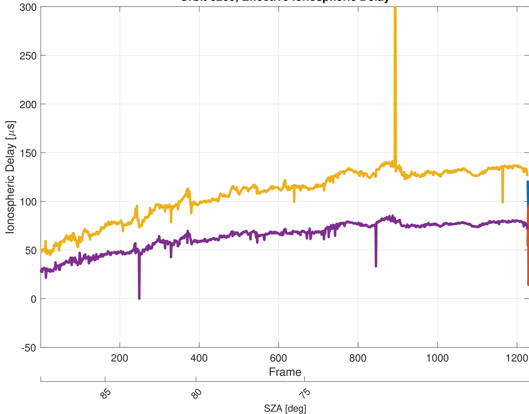
Orbit 6260, Effective Ionospheric Delay
