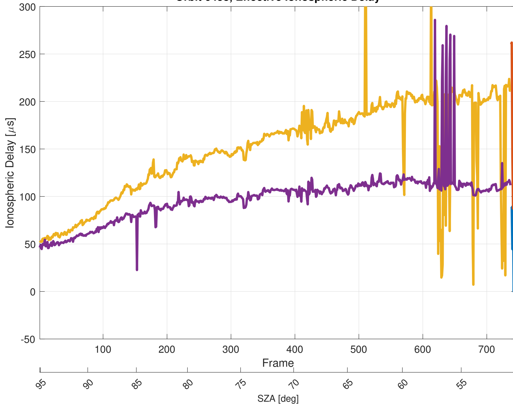
Orbit 6458, Effective Ionospheric Delay
