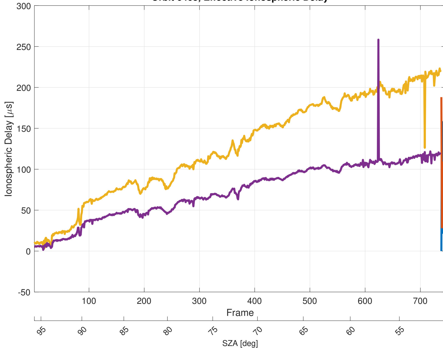
Orbit 6463, Effective Ionospheric Delay
