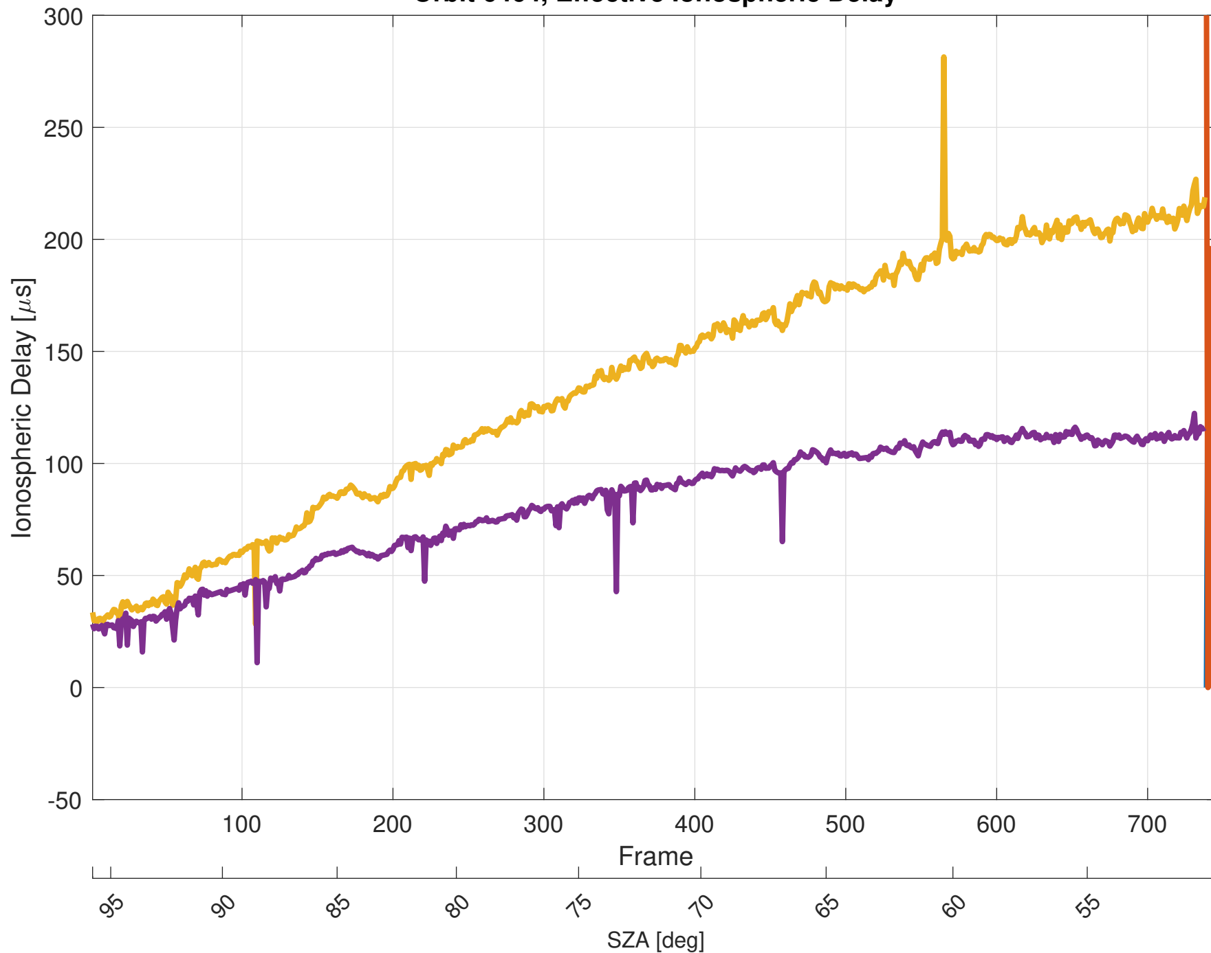
Orbit 6464, Effective Ionospheric Delay
