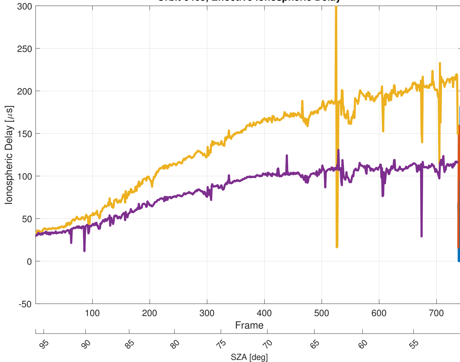
Orbit 6465, Effective Ionospheric Delay
