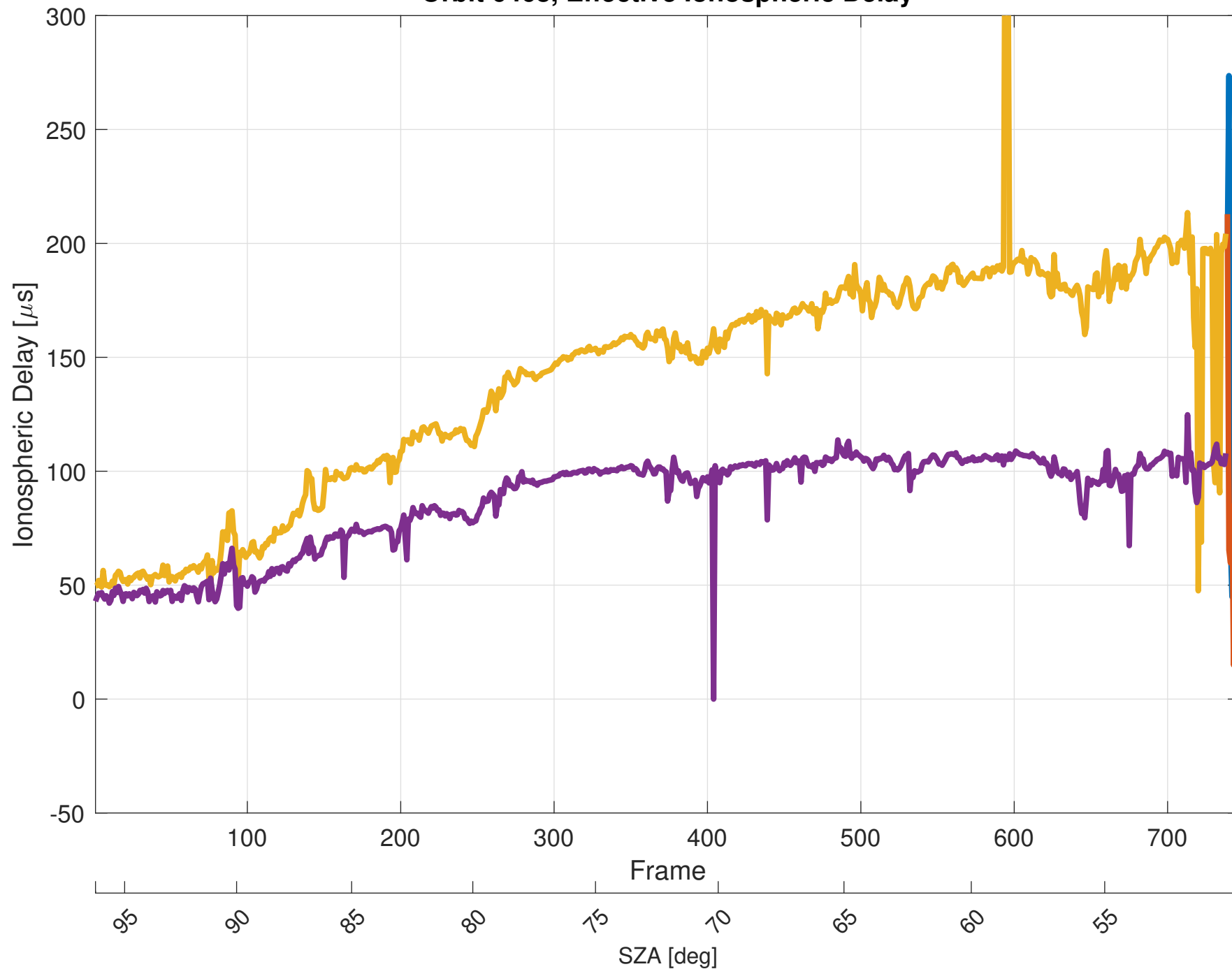
Orbit 6468, Effective Ionospheric Delay
