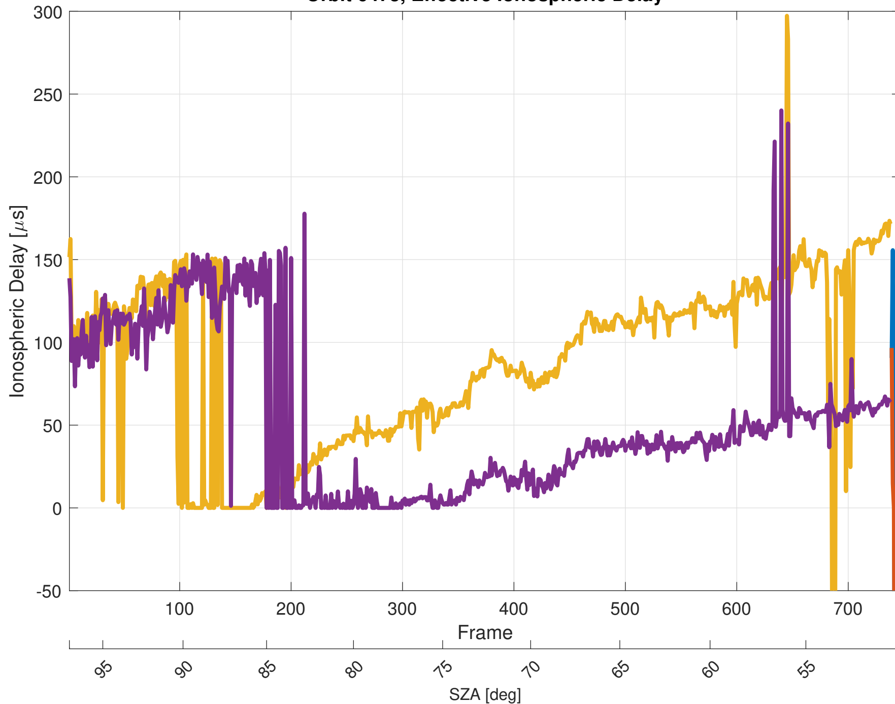
Orbit 6473, Effective Ionospheric Delay
