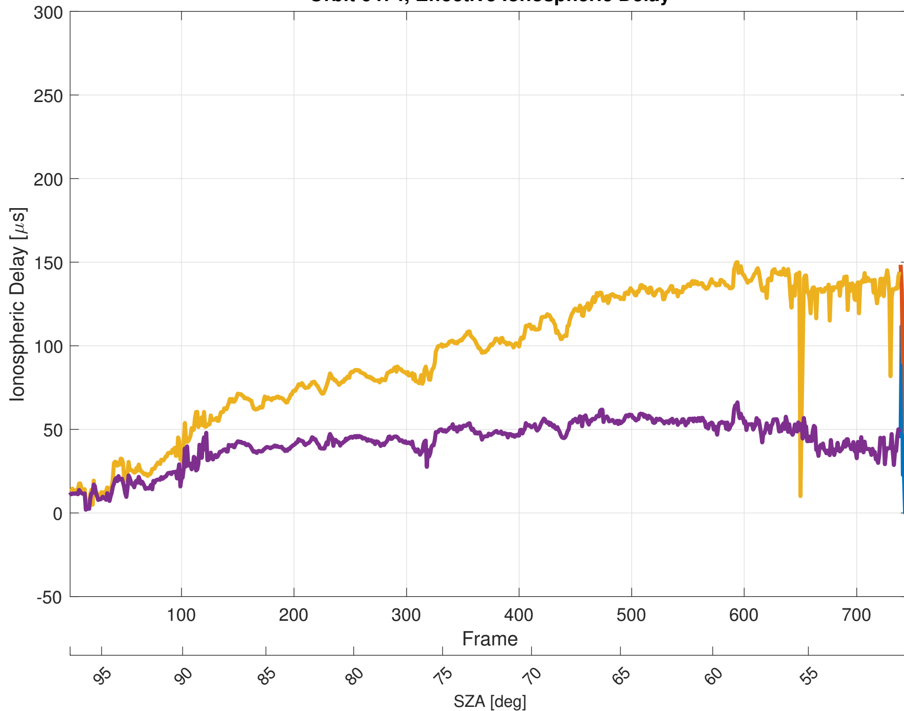
Orbit 6474, Effective Ionospheric Delay
