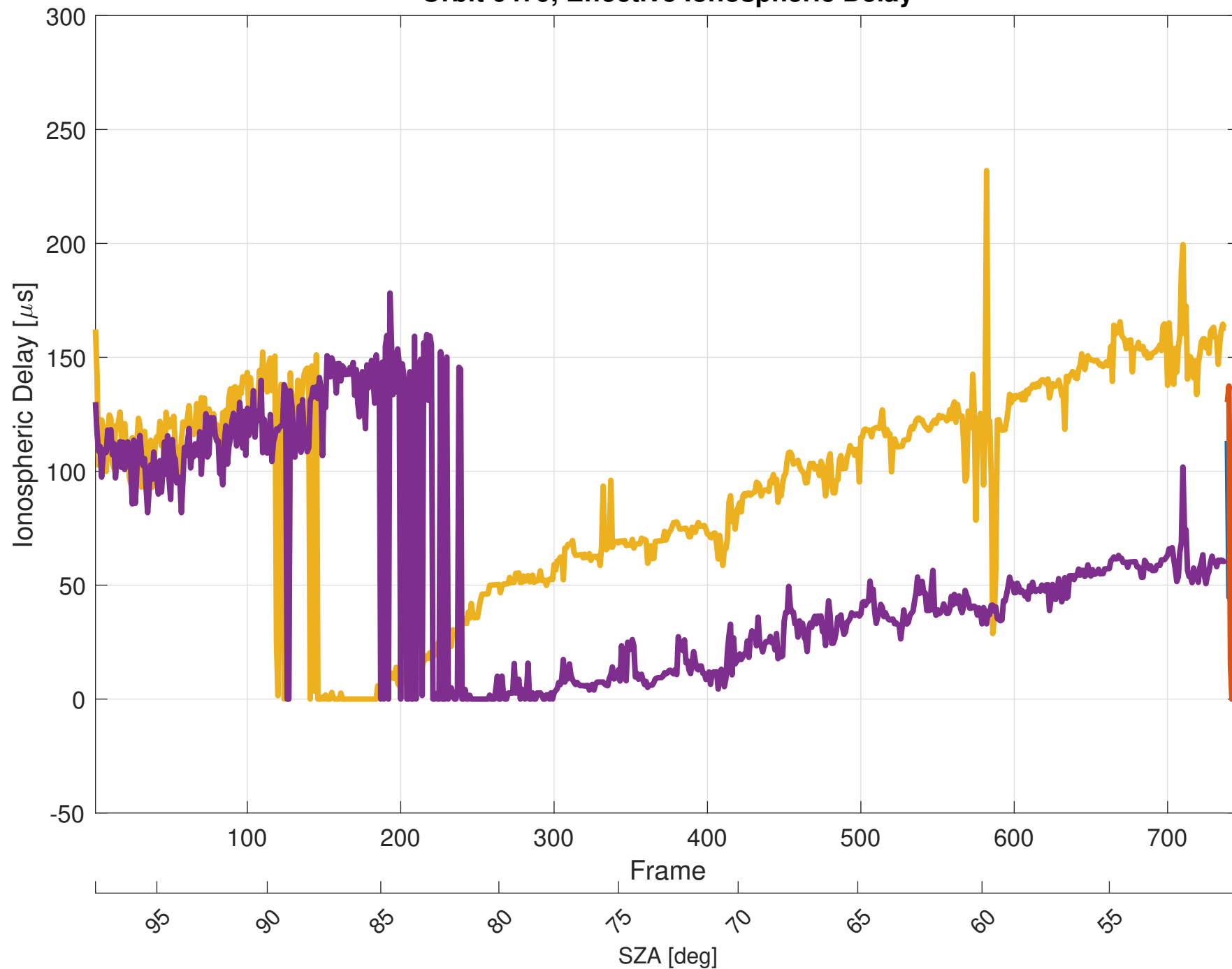
Orbit 6479, Effective Ionospheric Delay
