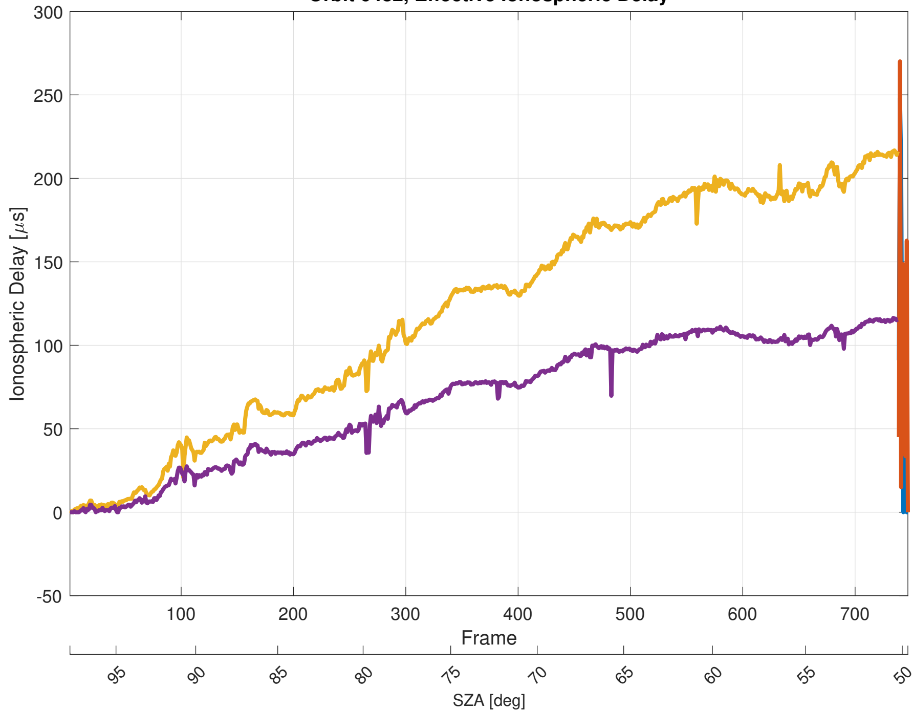
Orbit 6482, Effective Ionospheric Delay
