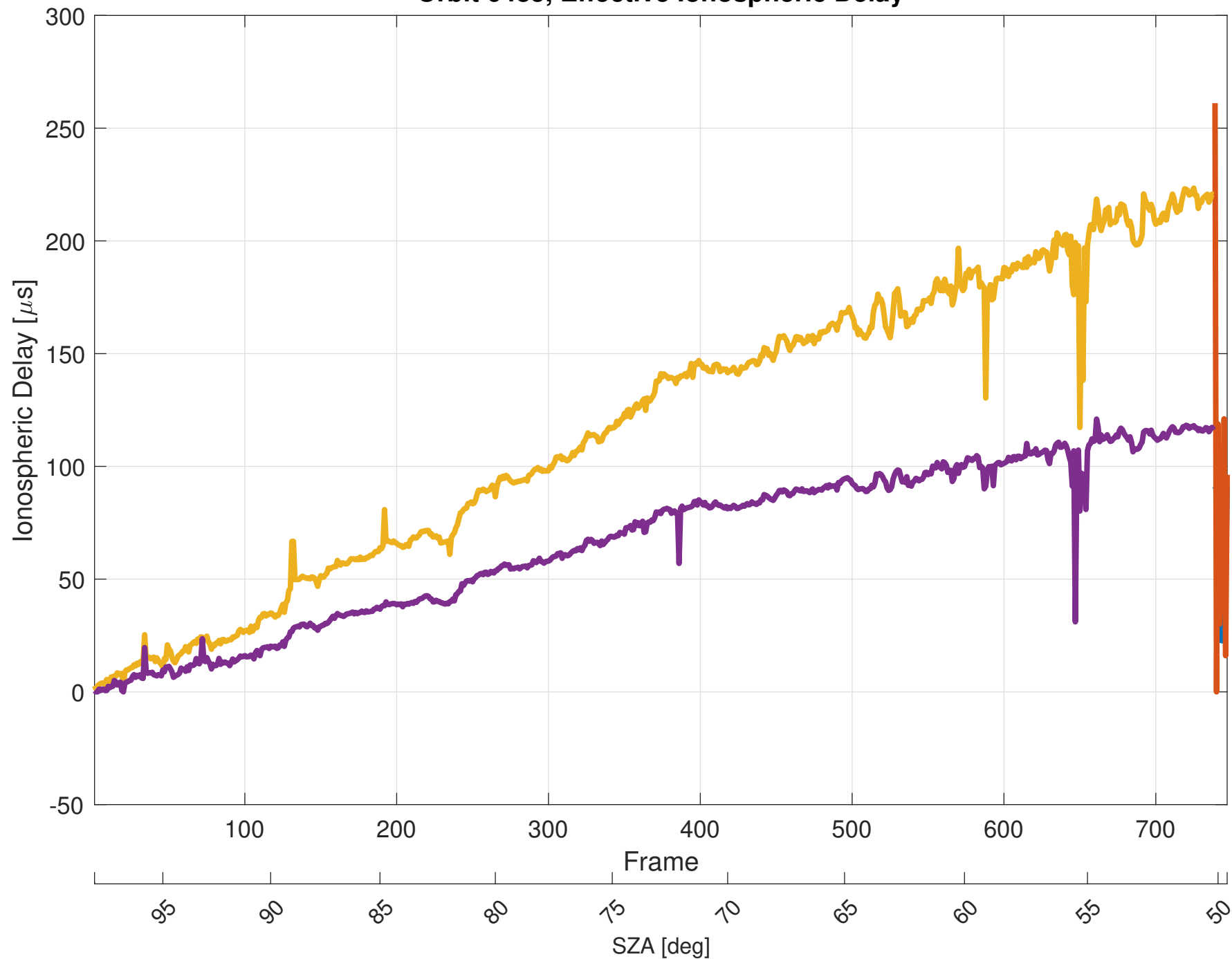
Orbit 6485, Effective Ionospheric Delay
