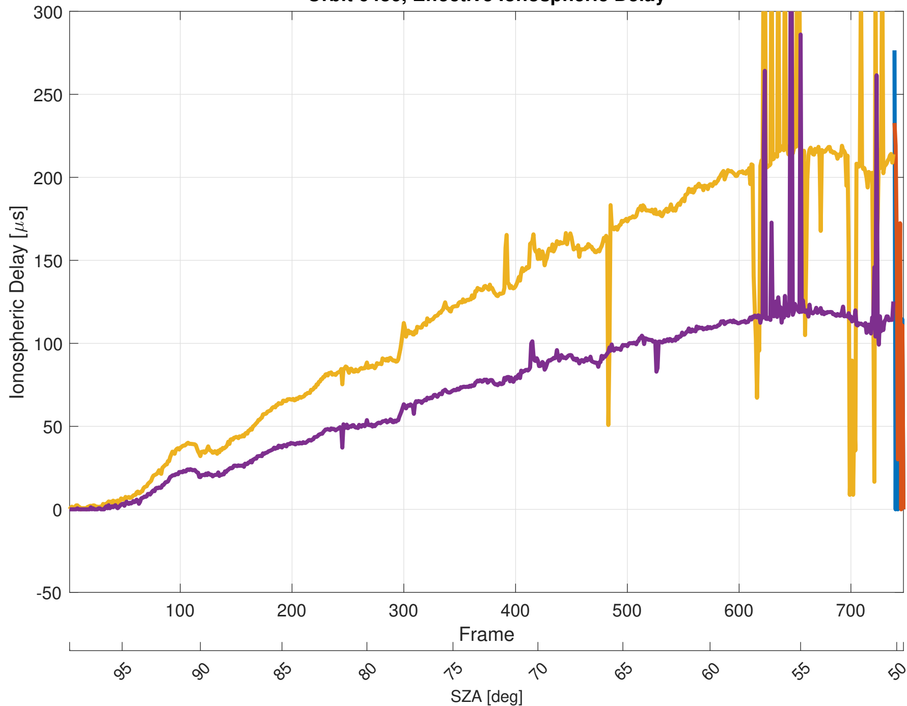
Orbit 6486, Effective Ionospheric Delay
