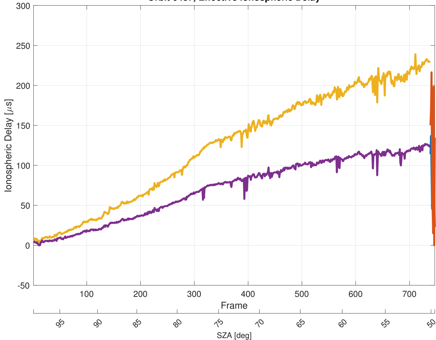
Orbit 6487, Effective Ionospheric Delay
