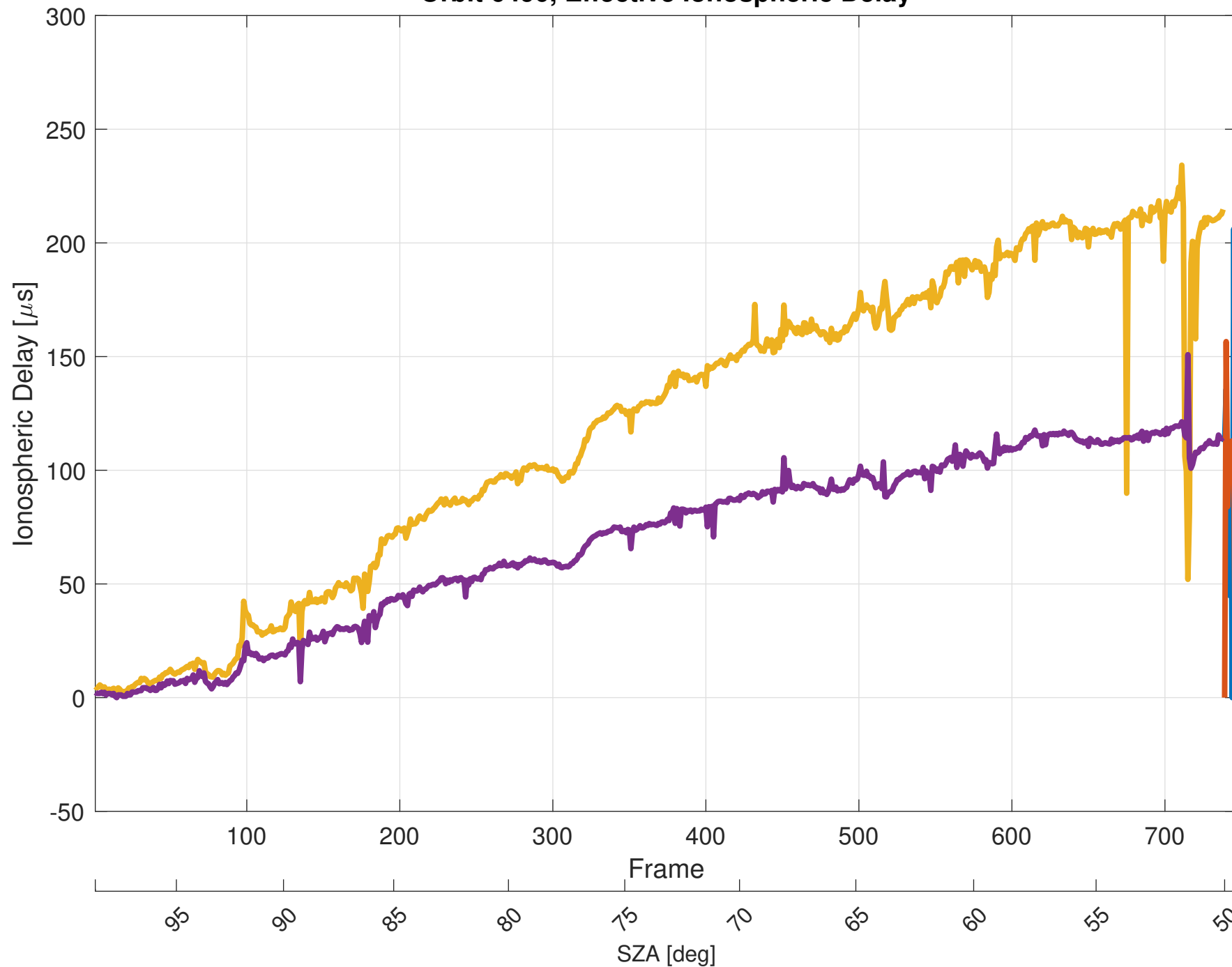
Orbit 6490, Effective Ionospheric Delay
