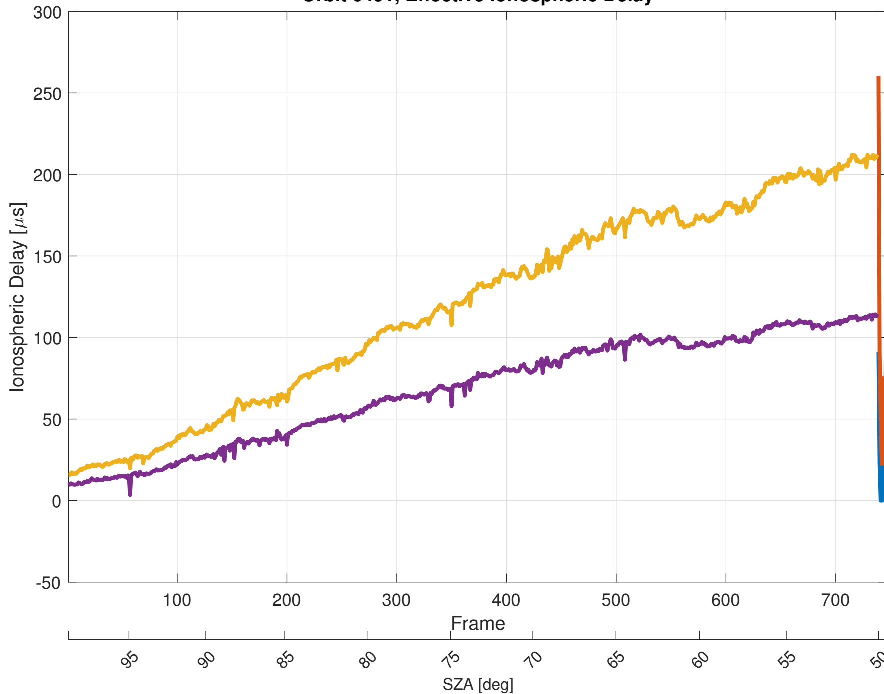
Orbit 6491, Effective Ionospheric Delay
