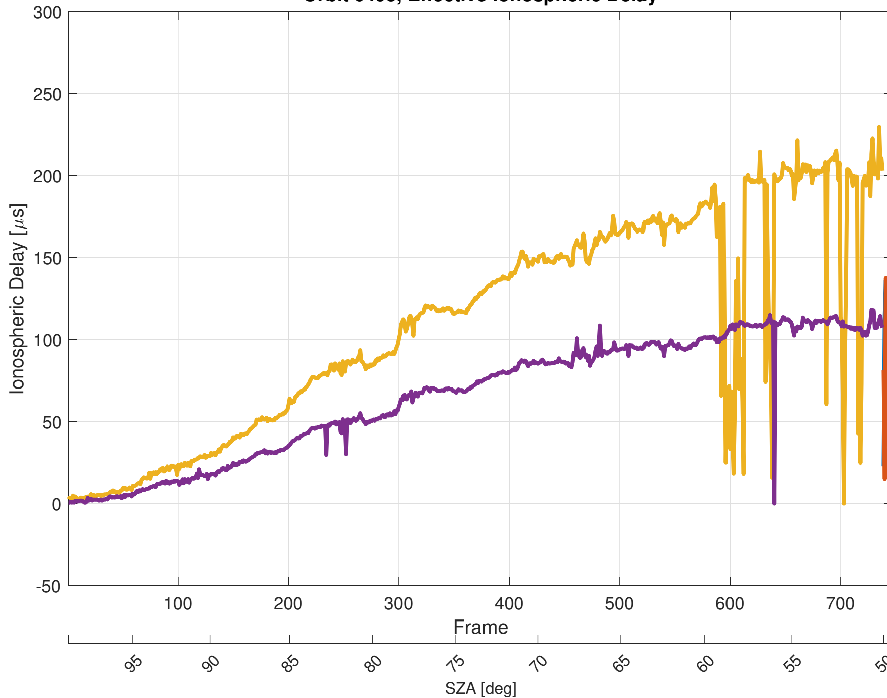
Orbit 6493, Effective Ionospheric Delay
