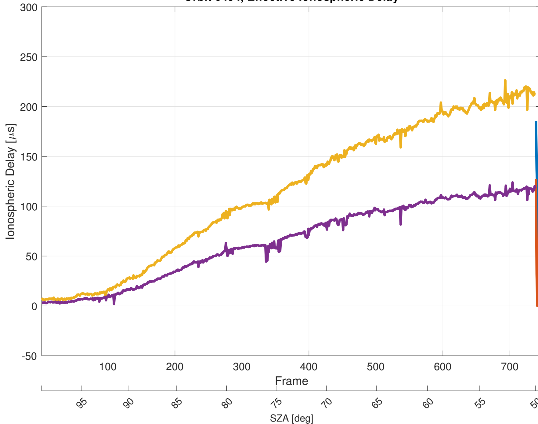
Orbit 6494, Effective Ionospheric Delay
