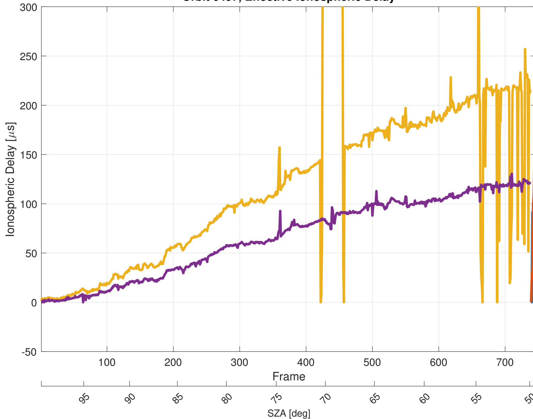
Orbit 6497, Effective Ionospheric Delay
