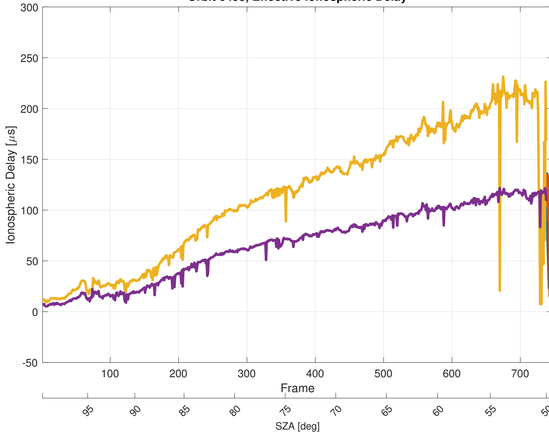
Orbit 6498, Effective Ionospheric Delay
