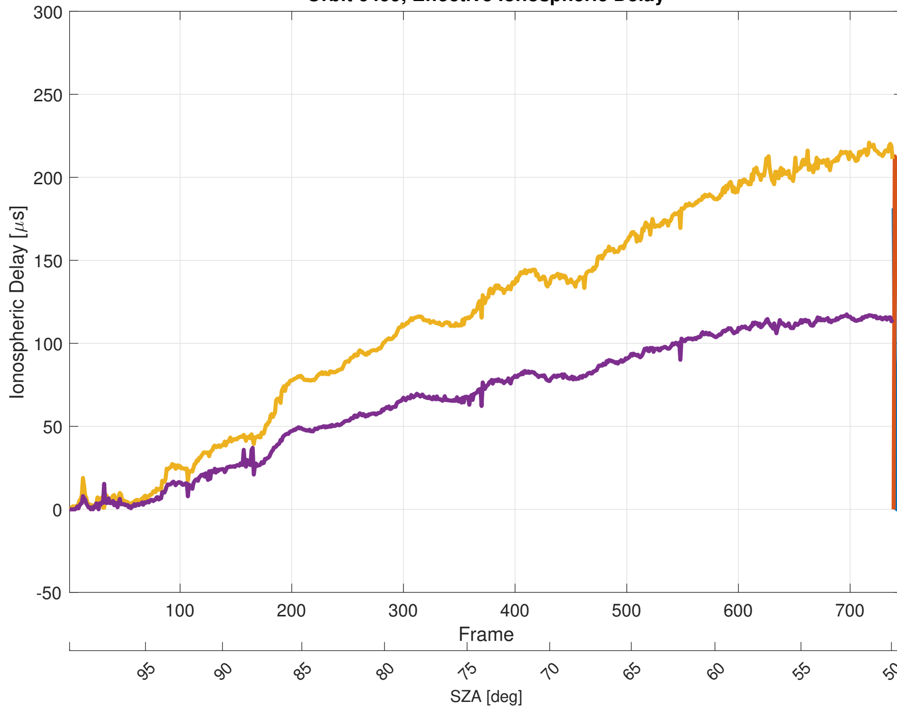
Orbit 6499, Effective Ionospheric Delay
