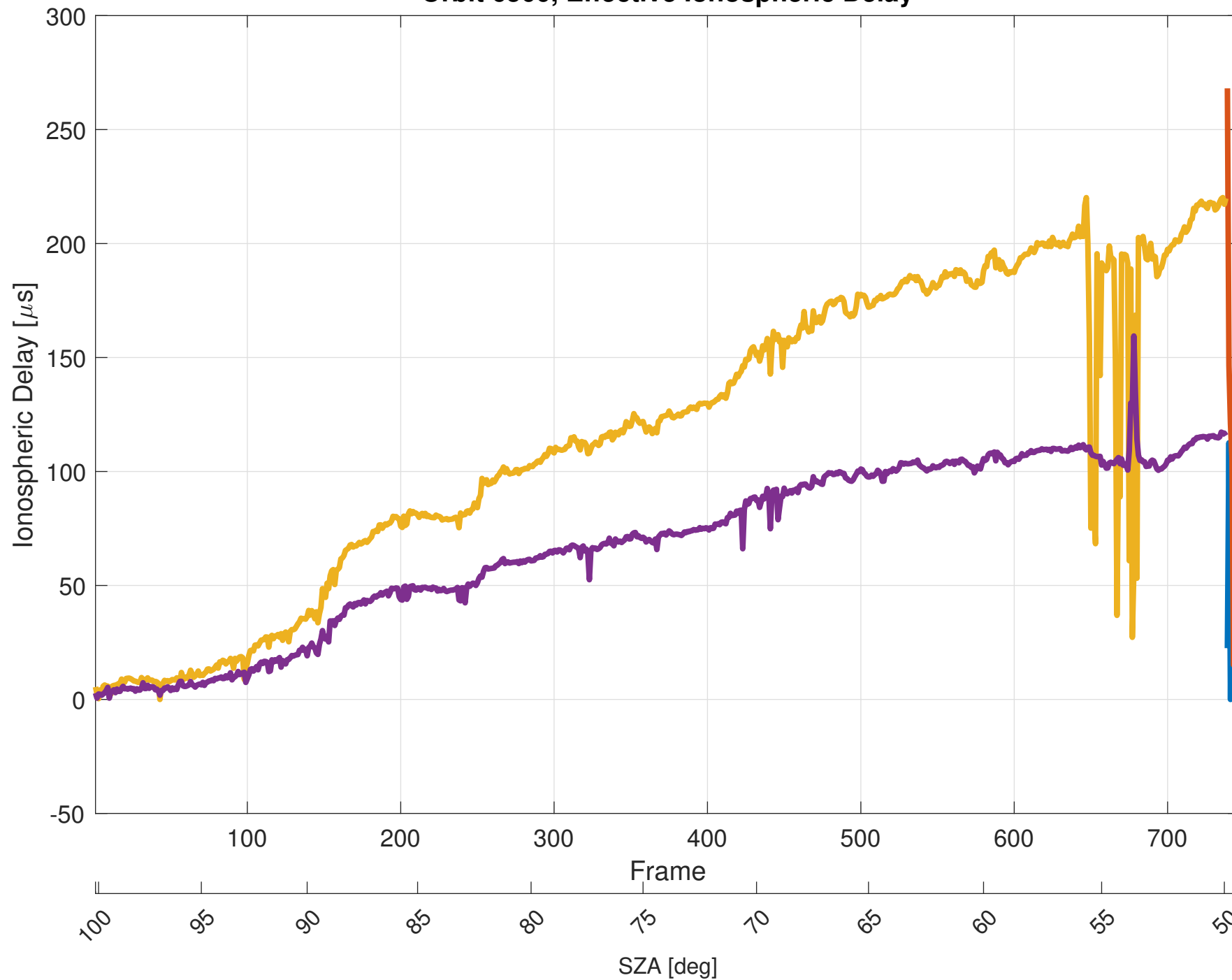
Orbit 6500, Effective Ionospheric Delay
