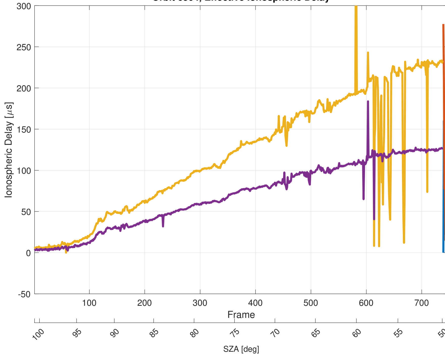
Orbit 6504, Effective Ionospheric Delay
