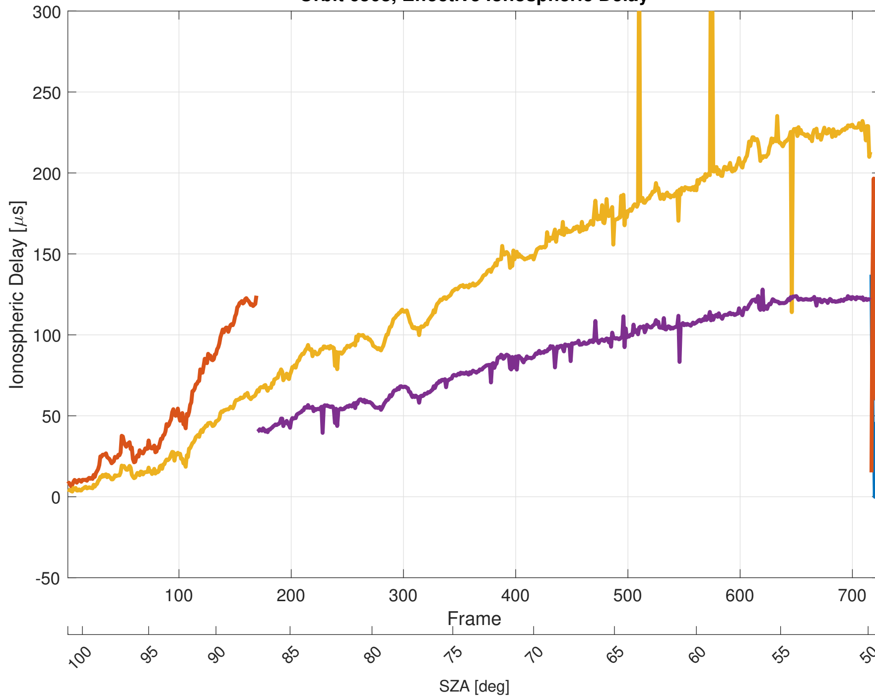
Orbit 6508, Effective Ionospheric Delay
