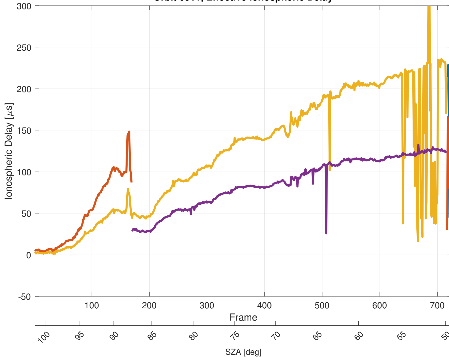
Orbit 6511, Effective Ionospheric Delay
