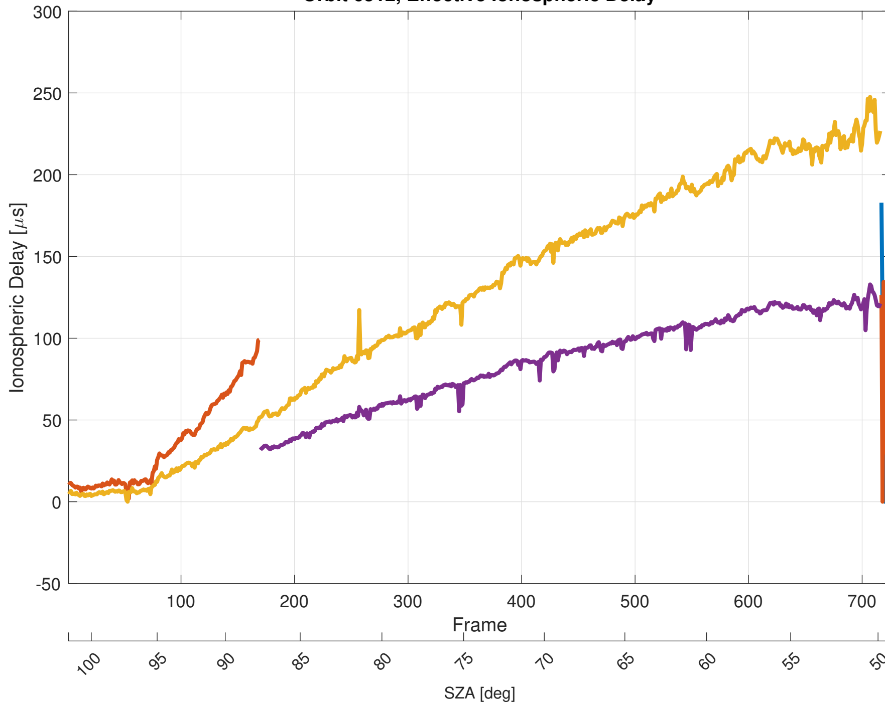
Orbit 6512, Effective Ionospheric Delay
