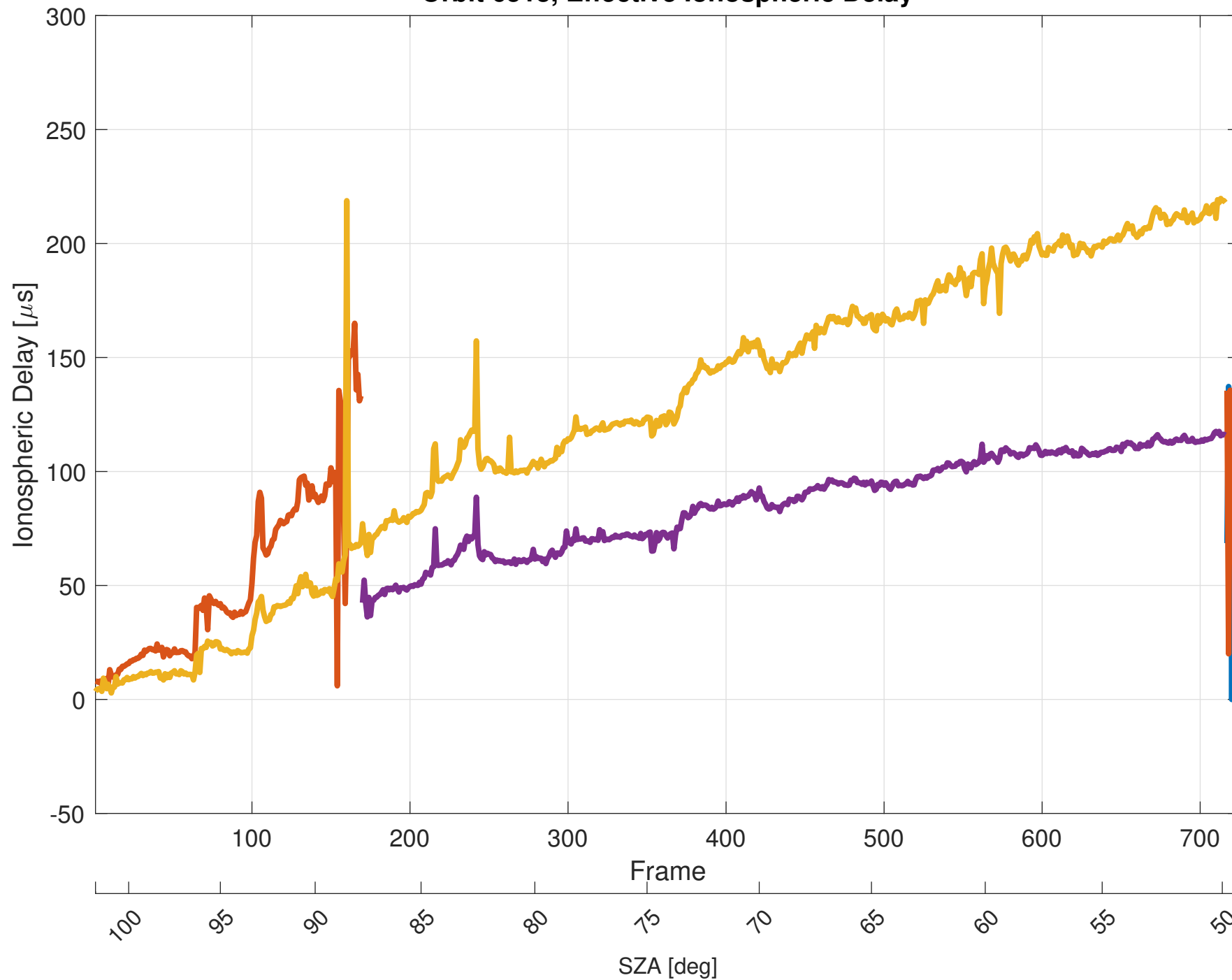
Orbit 6513, Effective Ionospheric Delay
