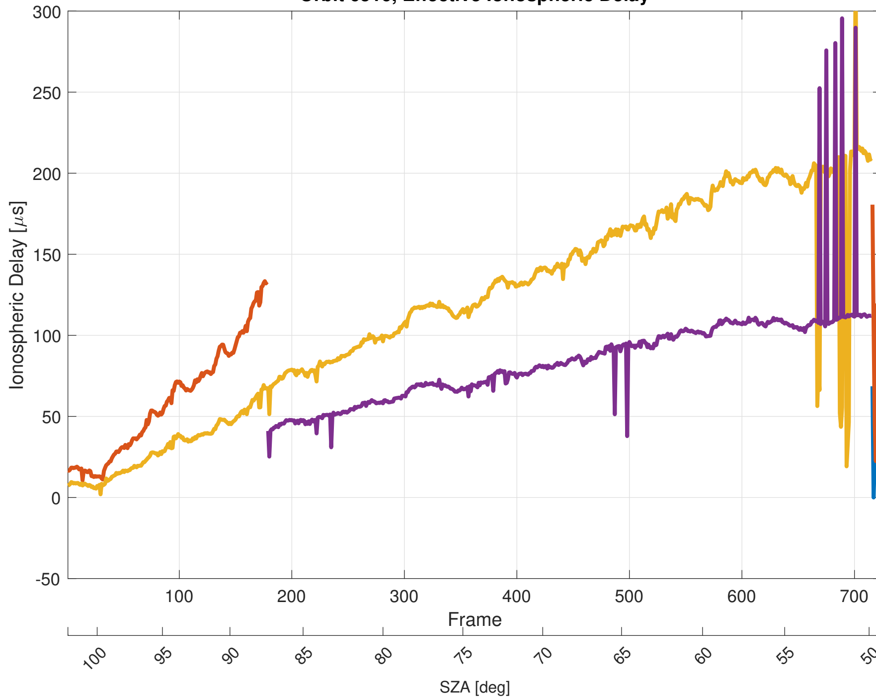
Orbit 6516, Effective Ionospheric Delay
