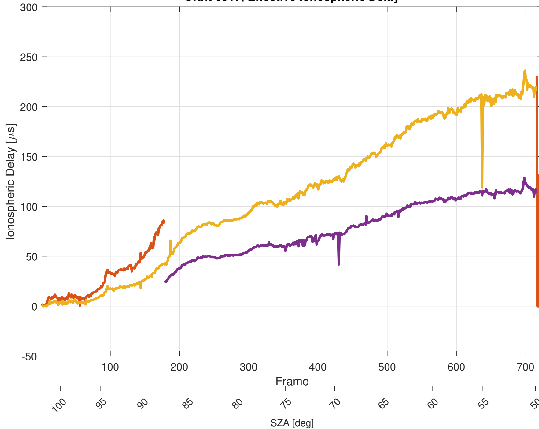
Orbit 6517, Effective Ionospheric Delay
