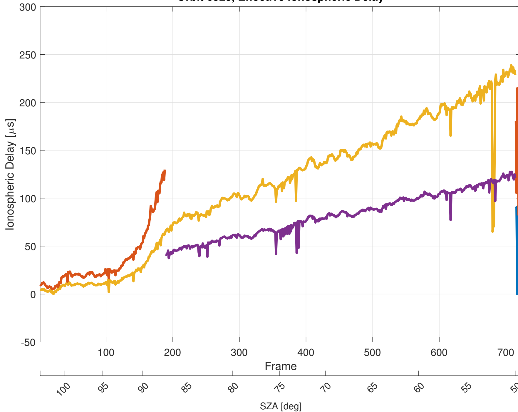
Orbit 6523, Effective Ionospheric Delay
