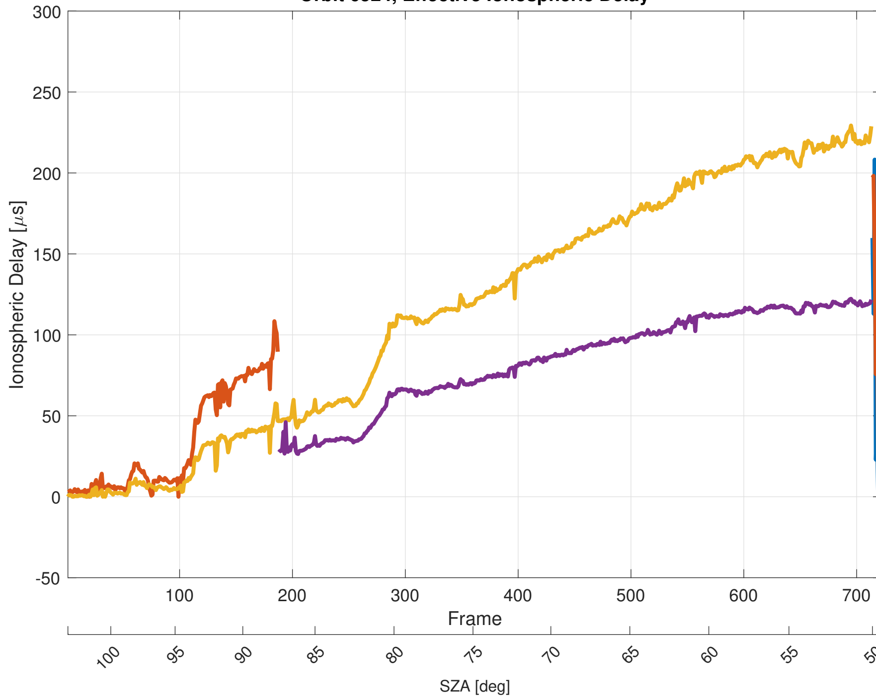
Orbit 6524, Effective Ionospheric Delay
